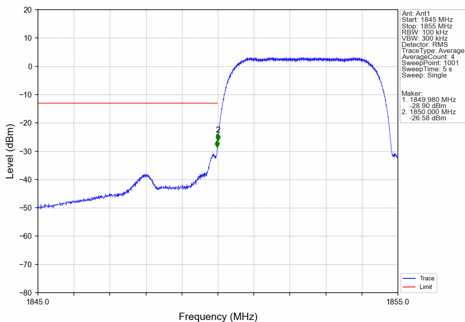
Band2_HSDPA_LCH_1852.4MHz_Subtest 1_NTNV
