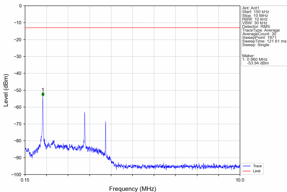
Band2_HSDPA_LCH_1852.4MHz_Subtest 1_NTV
