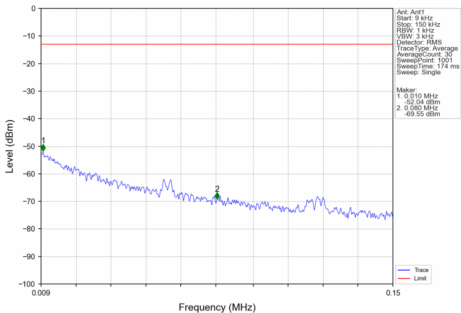
Band2_HSDPA_LCH_1852.4MHz_Subtest 1_NTV
