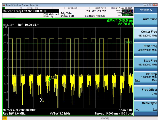
433.92 MHz: Period Time
