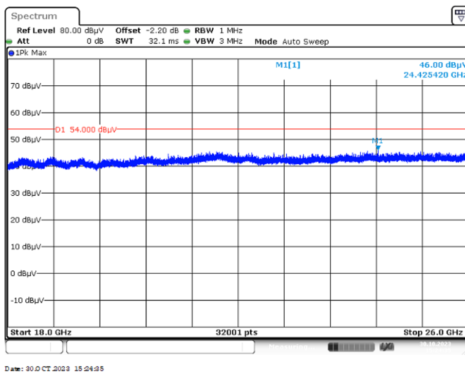
Plot 4: 18 GHz to 26 GHz, TX mode, vertical & horizontal polarization, 1 Msps, valid for all channels
