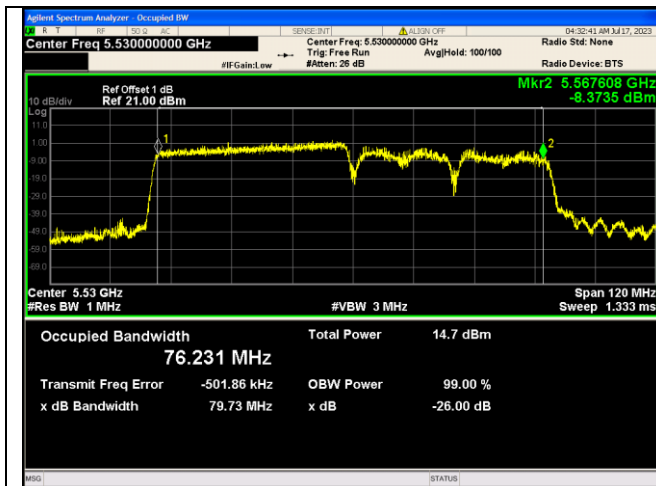
IEEE 802.11ax Channel 106 80MHz_Antenna 0 RU&Index 484RU65
