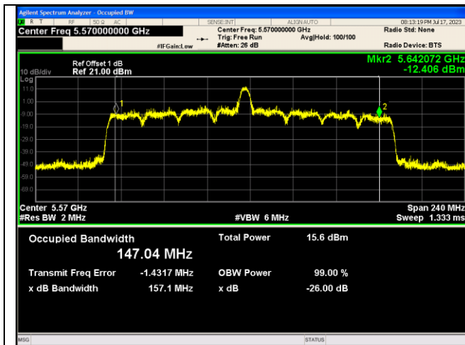
IEEE 802.11ax_Channel 114_160MHz_Antenna 0 RU&Index 52RU52
