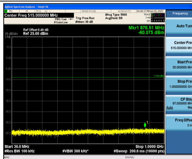
Band4-3MHz-QPSK-20385-1-0-Low-30-1000--60.08-PASS
