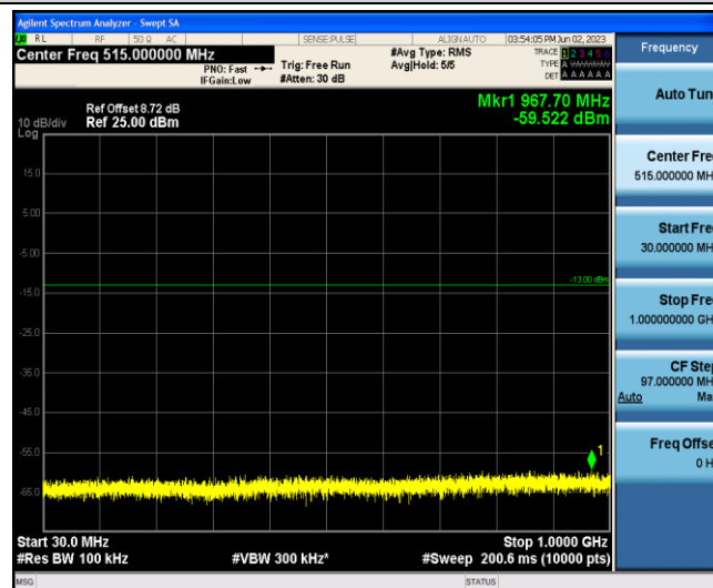
Band2-20MHz-16QAM-18900-1-0-Low-30-1000--59.52-PASS
