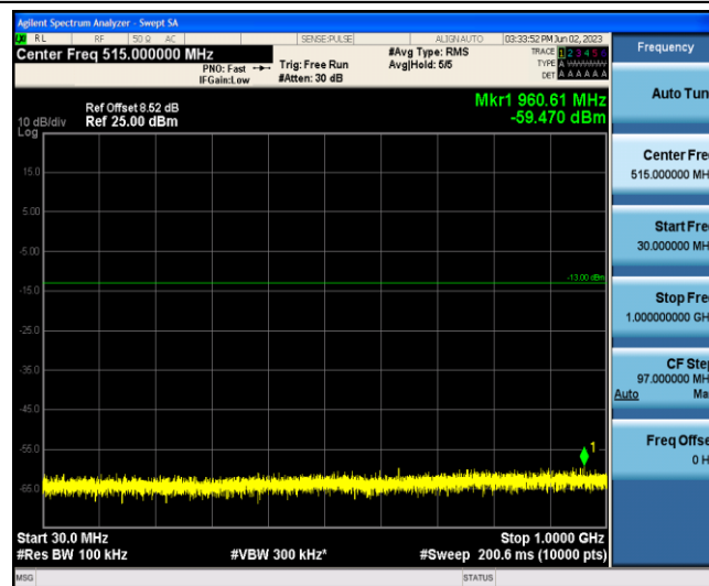
Band2-15MHz-16QAM-19125-1-0-Low-30-1000--59.47-PASS
