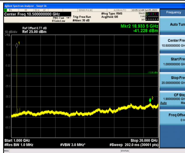
Band4-10MHz-QPSK-20000-1-0-Low-1000-20000--41.23-PASS
