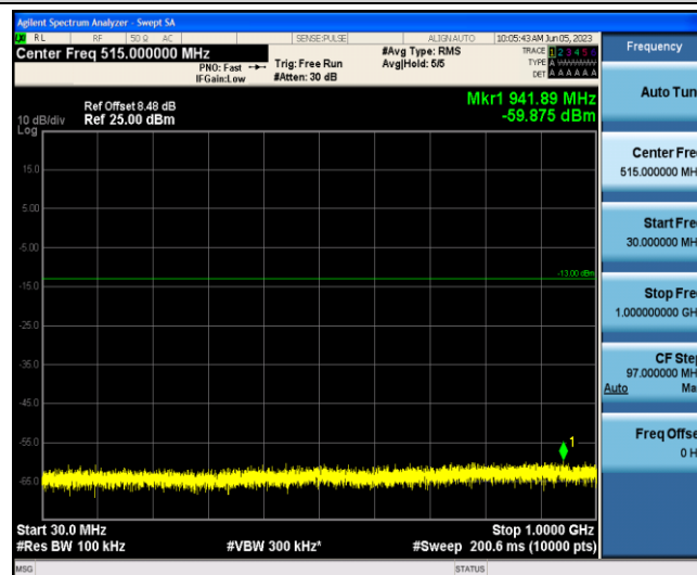
Band4-10MHz-QPSK-20175-1-0-Low-30-1000--59.88-PASS
