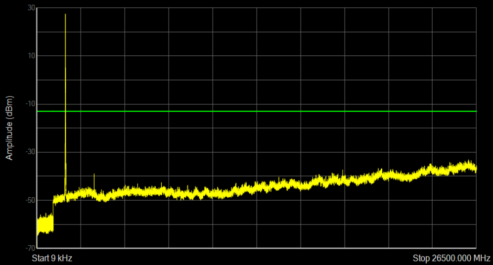
Band66 QAM16 BW=20MHz Channel=132322 RB Size=1 Position=#0
