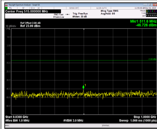
Band4-1.4MHz-64QAM-19957-1RB#0-Range1:30~1000MHz
