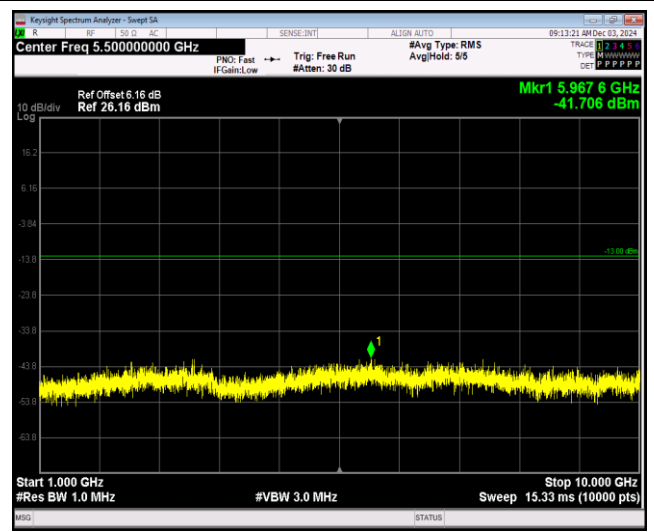
Band5-1.4MHz-16QAM-20407-1RB#0-Range2:1000~10000MHz
