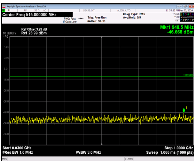
Band4-1.4MHz-16QAM-20175-1RB#0-Range1:30~1000MHz
