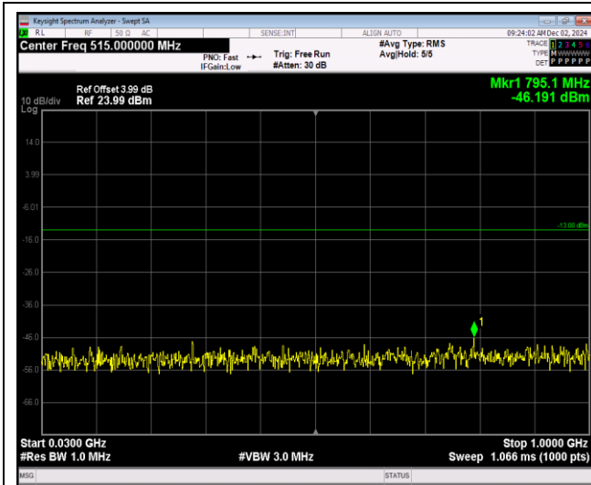
Band4-1.4MHz-QPSK-19957-1RB#0-Range1:30~1000MHz
