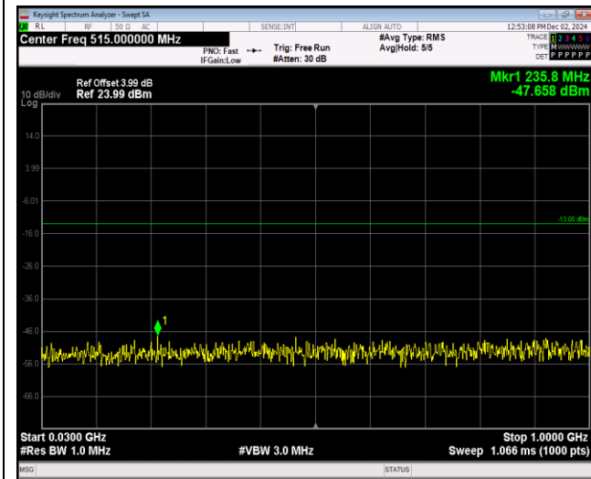
Band4-20MHz-QPSK-20300-1RB#0-Range1:30~100 OMHz
