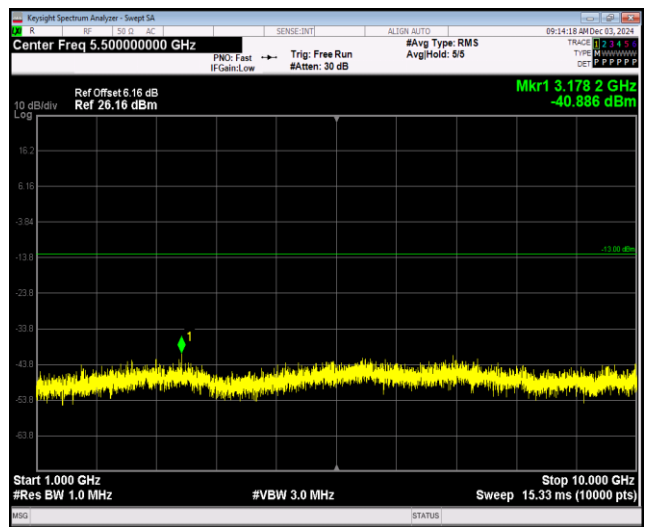
Band5-1.4MHz-16QAM-20643-1RB#0-Range2:1000 ~10000MHz
