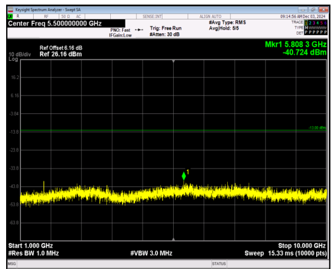
Band5-1.4MHz-16QAM-20407-1RB#0-Range2:1000~10000MHz
