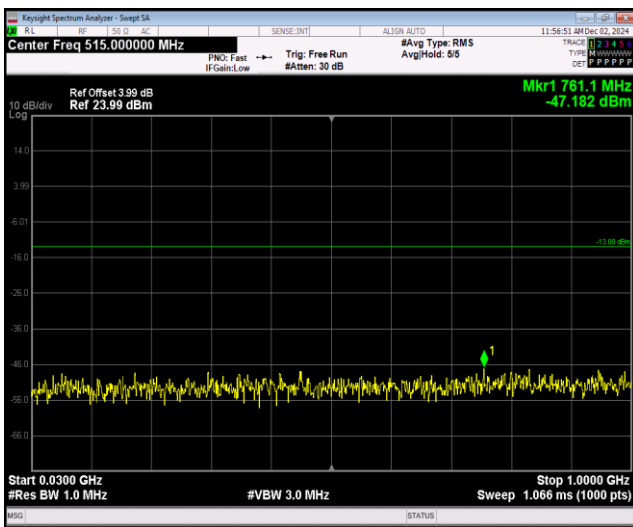
Band4-1.4MHz-16QAM-19957-1RB#0-Range1:30~1000MHz
