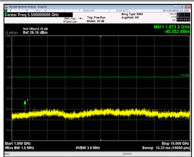
Band5-1.4MHz-QPSK-20643-1RB#0-Range2:1000~10000MHz
