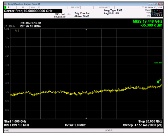
Band4-1.4MHz-64QAM-19957-1RB#0-Range2:1000~20000MHz
