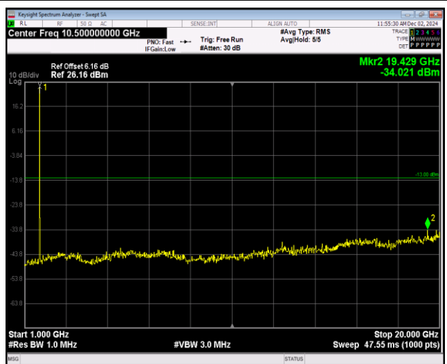
Band4-1.4MHz-16QAM-20175-1RB#0-Range2:1000~20000MHz
