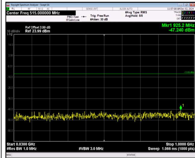
Band4-1.4MHz-64QAM-19957-1RB#0-Range1:30~1000MHz
