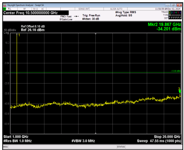
Band4-1.4MHz-16QAM-19957-1RB#0-Range2:1000~20000MHz
