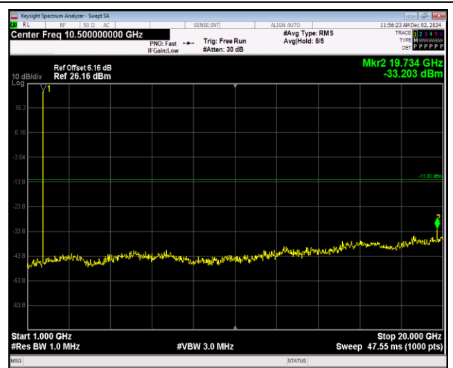
Band4-1.4MHz-16QAM-20393-1RB#0-Range2:1000~20000MHz
