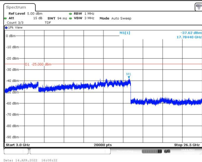
Band38-20MHz-16QAM-38150-100RB#0-Range3:3000~26500MHz
