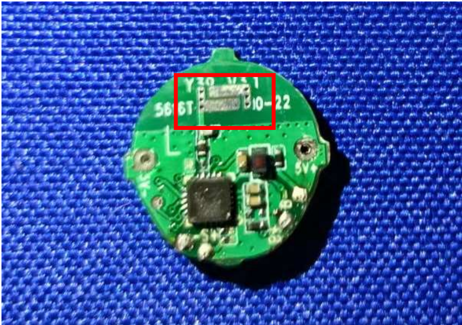
BT Antenna
