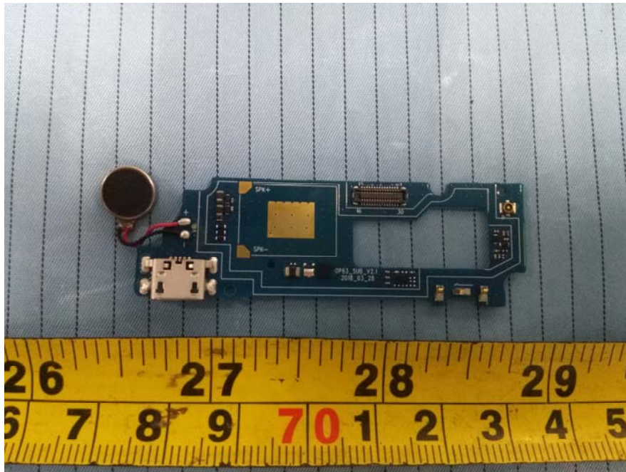
EUT – Small Board Top Shielding off View
