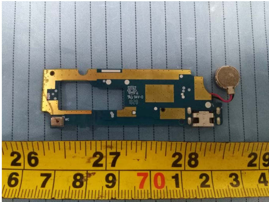
EUT – Small Board Bottom Shielding off View
