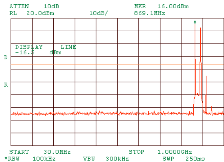
Plot 1.7.45 Spurious emission measurements in 30 - 1000 MHz range at low carrier frequency OFDM
