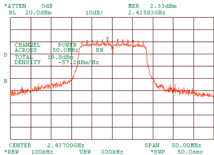
Plot 1.5.10 Peak output power at mid frequency of MA 850 and MA 1000 interconnected, port 1. At 12Mbps OFDM.
