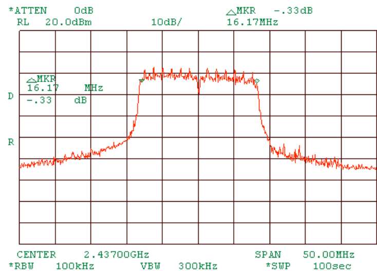
Plot 1.2.29 6 dB bandwidth test result at mid frequency of MA 850 stands alone. At 24 Mbps OFDM.
