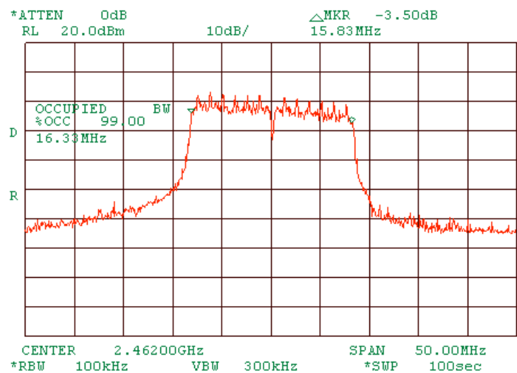
Plot 1.2.40 99 power bandwidth test result at high frequency of MA 850 stands alone. At 54 Mbps OFDM.
