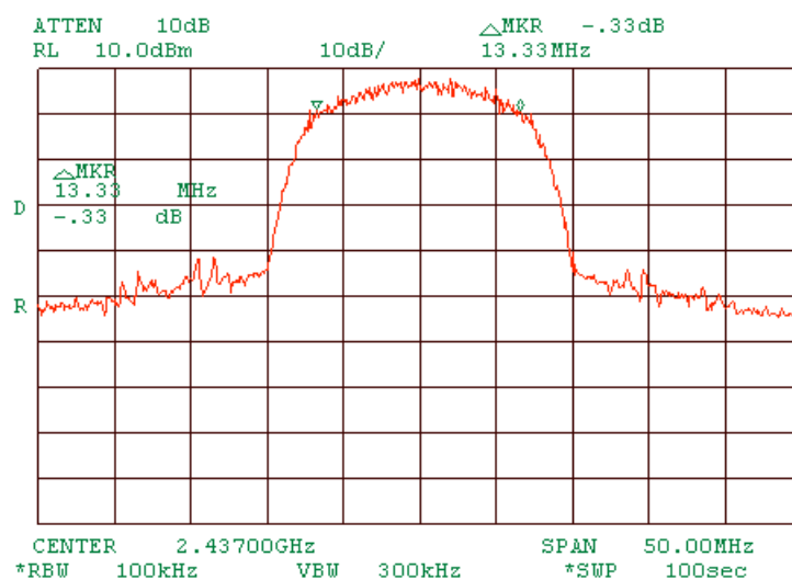
Plot 1.1.7 6 dB bandwidth test result at mid frequency with MA 850 and MA 1000 interconnected. At 11 Mbps DSSS.
