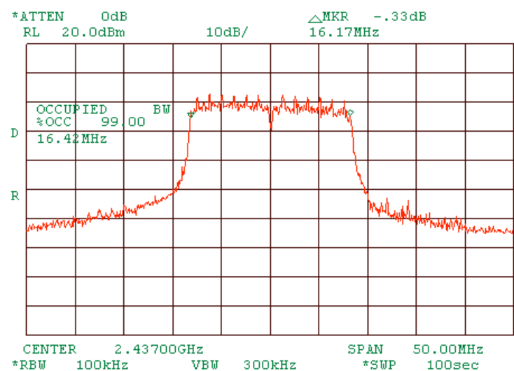
Plot 1.2.30 99% power bandwidth test result at mid frequency of MA 850 stands alone. At 24 Mbps OFDM.
