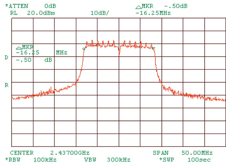
Plot 1.2.27 6 dB bandwidth test result at mid frequency of MA 850 stands alone. At 18 Mbps OFDM.
