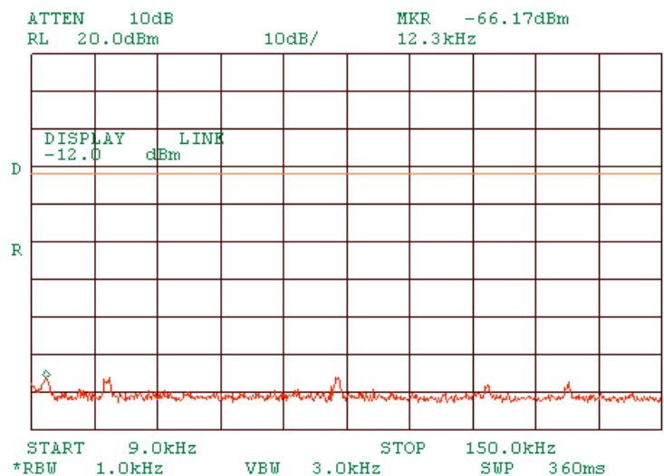
Plot 1.7.5 Spurious emission measurements in 9 - 150 kHz range at mid carrier frequency DSSS
