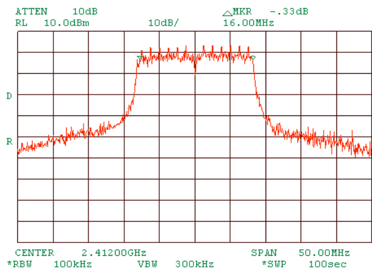
Plot 1.1.16 99% power bandwidth test result at low frequency with MA 850 and MA 1000 interconnected. At 54 Mbps OFDM.
