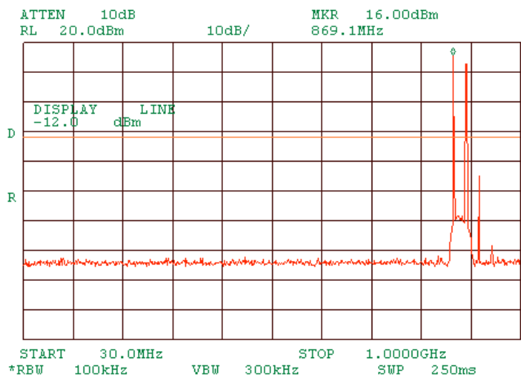
Plot 1.7.14 Spurious emission measurements in 30 - 1000 MHz range at high carrier frequency DSSS
