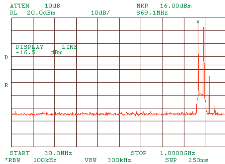
Plot 1.7.47 Spurious emission measurements in 30 - 1000 MHz range at mid carrier frequency OFDM
