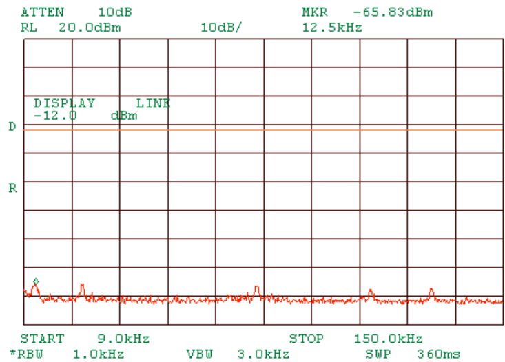
Plot 1.7.6 Spurious emission measurements in 9 - 150 kHz range at high carrier frequency DSSS
