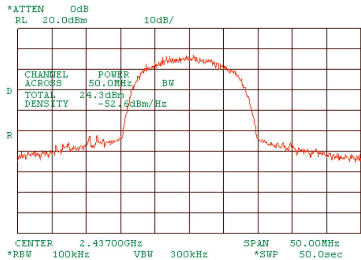
Plot 1.4.14 Peak output power at mid frequency of MA 850 and MA 1000 interconnected, port 3. At 5.5 Mbps DSSS.
