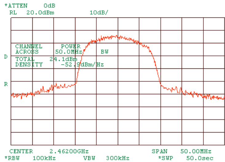
Plot 1.6.21 Peak output power at high frequency of MA 850, port 4. At 5.5Mbps DSSS.
