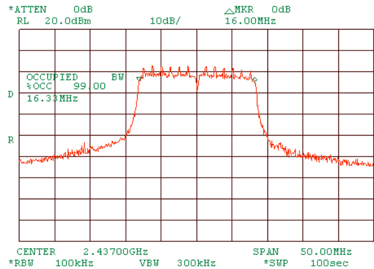
Plot 1.2.28 99% power bandwidth test result at mid frequency of MA 850 stands alone. At 18 Mbps OFDM.
