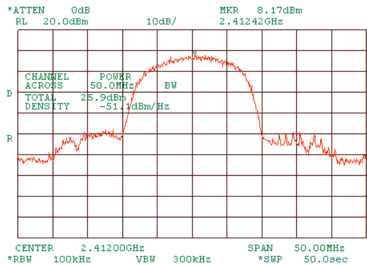
Plot 1.6.1 Peak output power at low frequency of MA 850, port 1. At 5.5Mbps DSSS.
