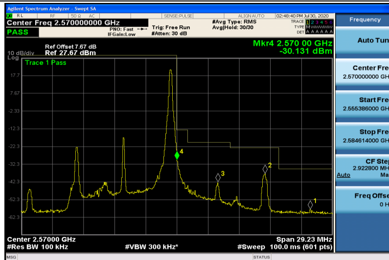
Band7-10MHz-QPSK-21400-1RB#49
