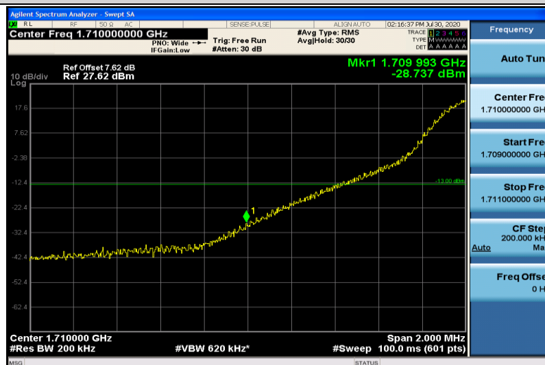
Band4-20MHz-16QAM-20050-1RB#0
