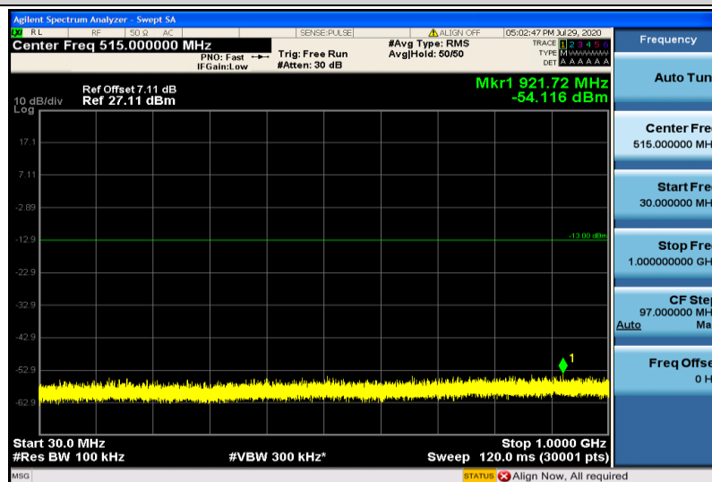
Band2-1.4MHz-QPSK-18900-1RB#0-30~1000MHz
