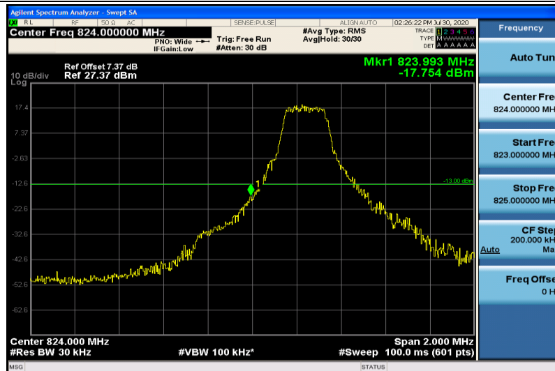
Band5-3MHz-16QAM-20415-1RB#0
