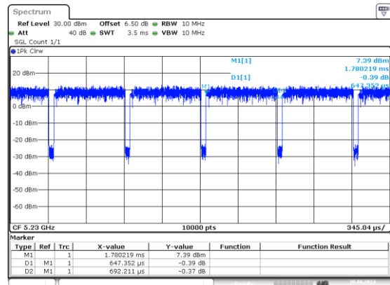
n40_5230MHz_Chain 1 0.647ms,0.692ms
