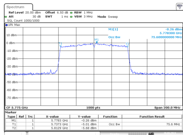
ac80_5775MHz_Chain 1 75.600MHz
