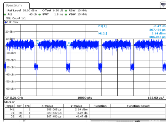
802.11ac80_5210MHz_Chain 1 0.324ms,0.367ms
