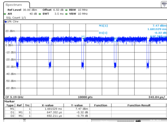
n40_5190MHz_Chain 1 0.647ms,0.692ms
