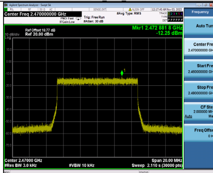
16QAM Ant2_2470
