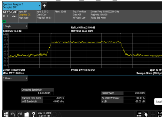
B4_N2(5M)_CP-OFDM_64 QAM_Outer_Full_Mid_CH
