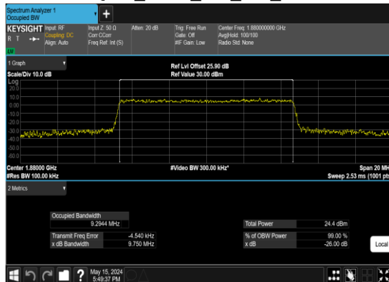
B4_N2(10M)_CP-OFDM_64 QAM_Outer_Full_Mid_CH
