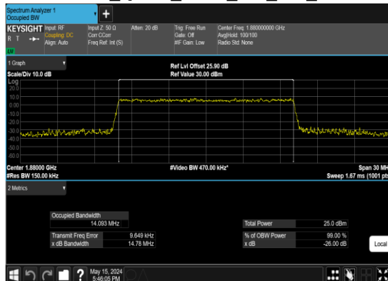
B4_N2(15M)_CP- OFDM_QPSK_Outer_Full_Mid_CH
