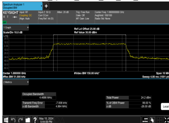
B4_N2(5M)_CP- OFDM_QPSK_Outer_Full_Mid_CH
