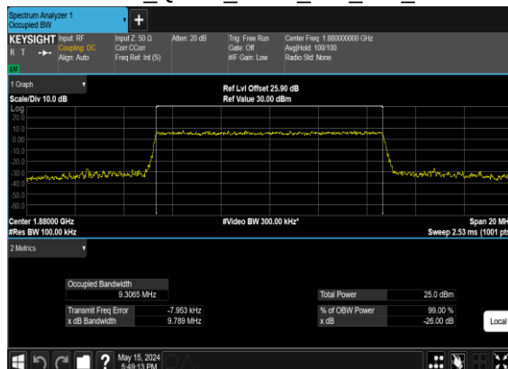
B4_N2(10M)_CP- OFDM_QPSK_Outer_Full_Mid_CH
