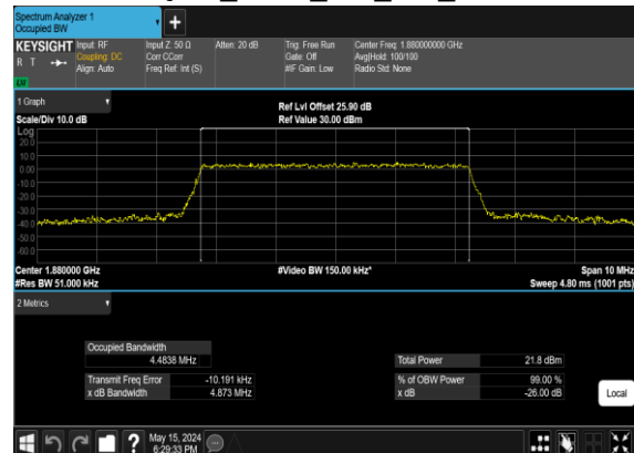
B4_N2(5M)_CP-OFDM_256 QAM_Outer_Full_Mid_CH
