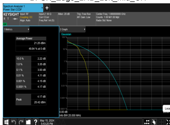
B4_N2(20M)_DFT-s-OFDM_PI_2-BPSK_Edge_1RB_Left_Mid_CH
