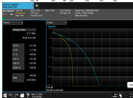
B4_N2(20M)_DFT-s-OFDM_QPSK_Edge_1RB_Left_Mid_CH
