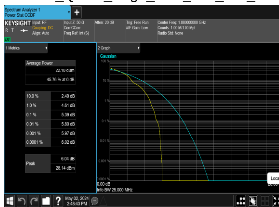
N2(20M)_DFT-s-OFDM_QPSK_Edge_1RB_Left_Mid_CH
