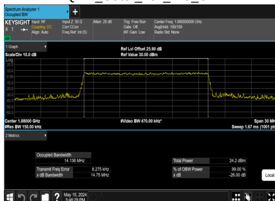
B4_N2(15M)_CP-OFDM_64 QAM_Outer_Full_Mid_CH
