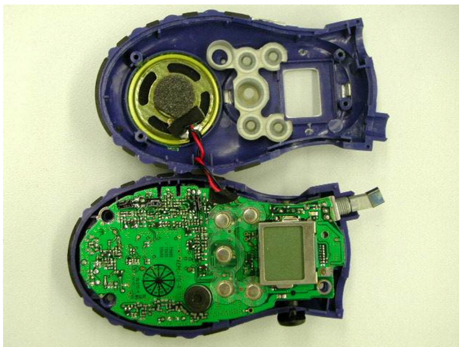
Internal Photo (T5900) – 4
