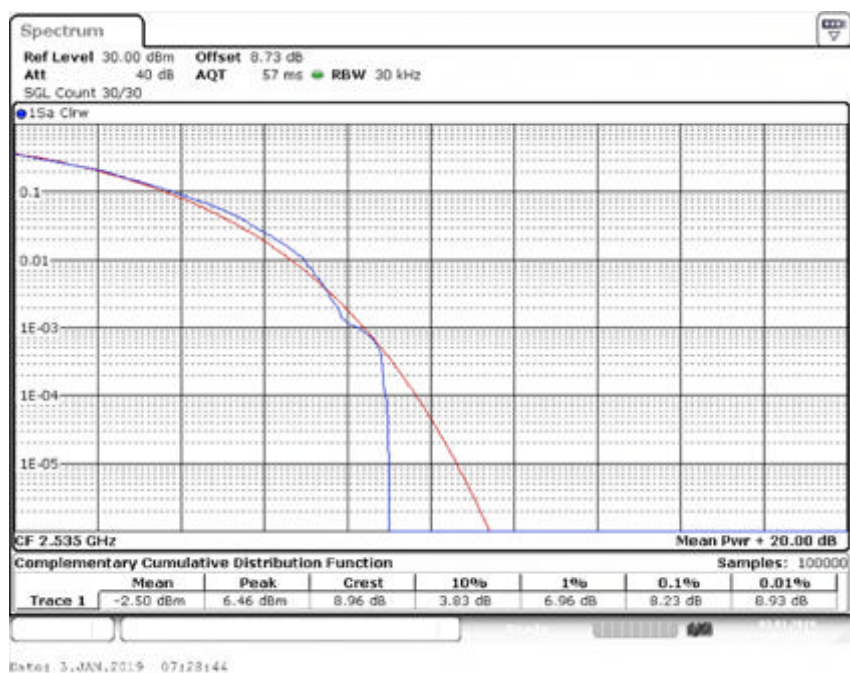
Peak-Average Ratio Plot(10MHz BW,QPSK,Band 7-mid Channel)
