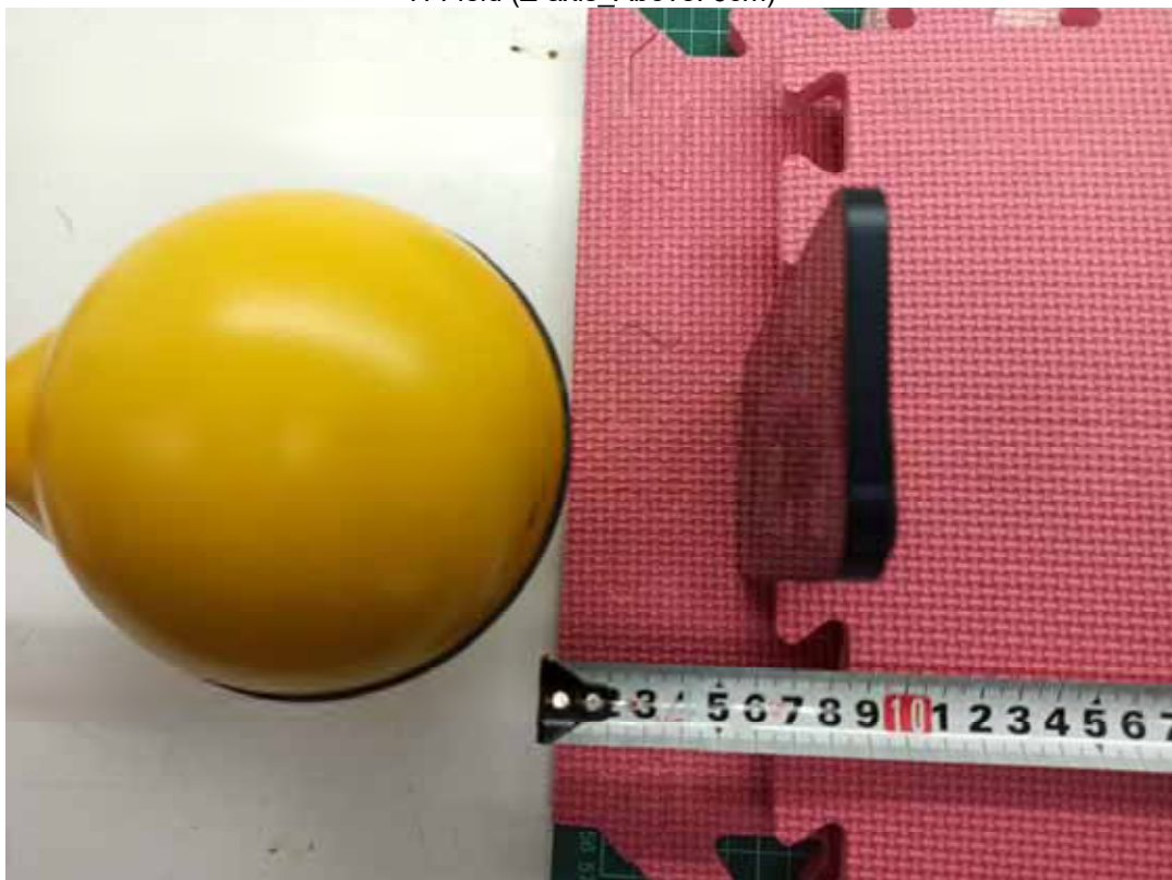
H-Field (Z-axis_Below: 6cm)
