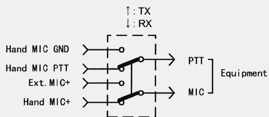
PTT / Ext. MIC Switch Circuit
