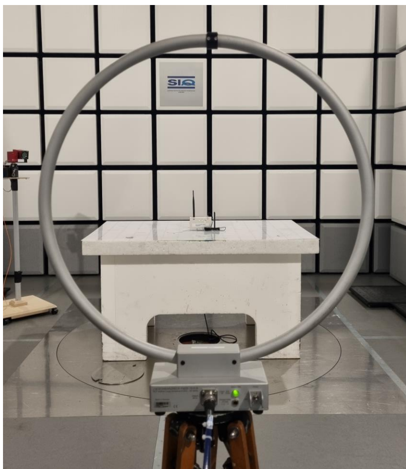
Figure 2: Spurious emission 90 kHz-30 MHz
