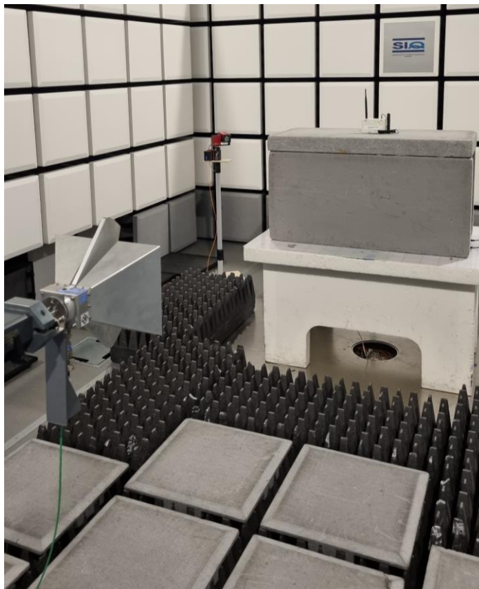
Figure 4: Spurious emission 1-18 GHz
