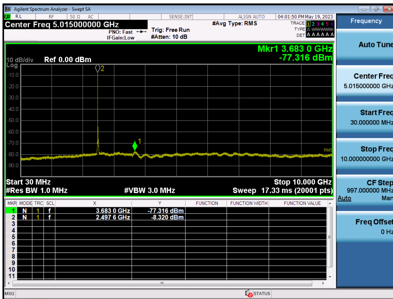
LTE41_20 M_CSE(30 M-10 G)_Lowest Channel
