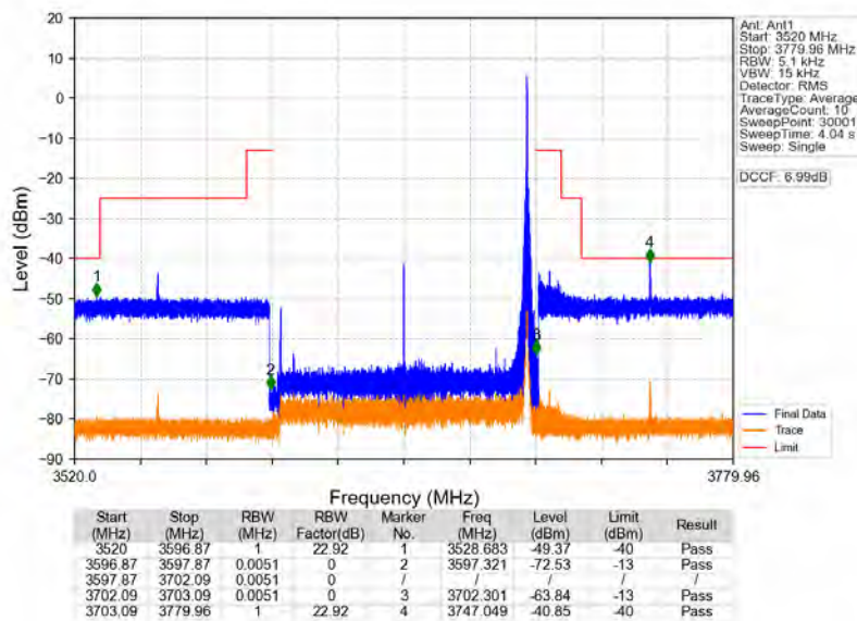
n78d_30kHz_MIMO_NTNV_100MHz_CP-OFDM_QPSK_3649.98MHz_Inner_1RB_Right
