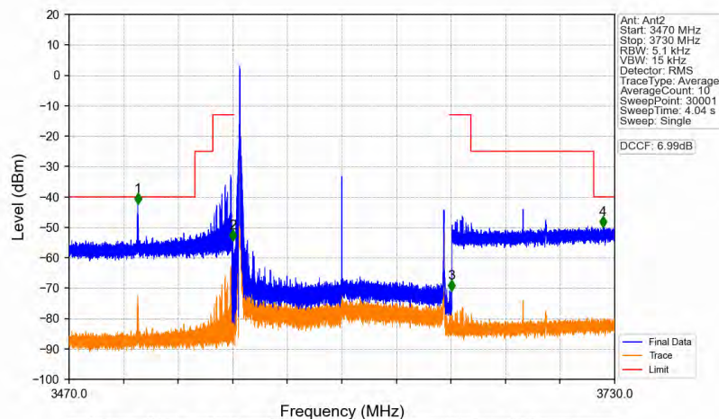
n78d_30kHz_MIMO_NTNV_100MHz_CP-OFDM_QPSK_3600MHz_Inner_1RB_Left
