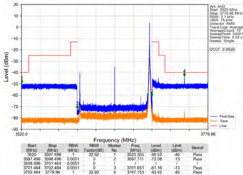
n78d_30kHz_MIMO_NTNV_100MHz_CP-OFDM_QPSK_3649.98MHz_Inner_1RB_Right
