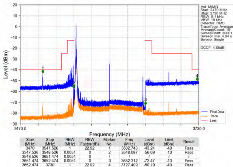
n78d_30kHz_MIMO_NTNV_100MHz_CP-OFDM_QPSK_3600MHz_Inner_1RB_Left
