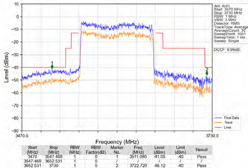
n78d_30kHz_MIMO_NTNV_100MHz_CP-OFDM_QPSK_3600MHz_Outer_Full
