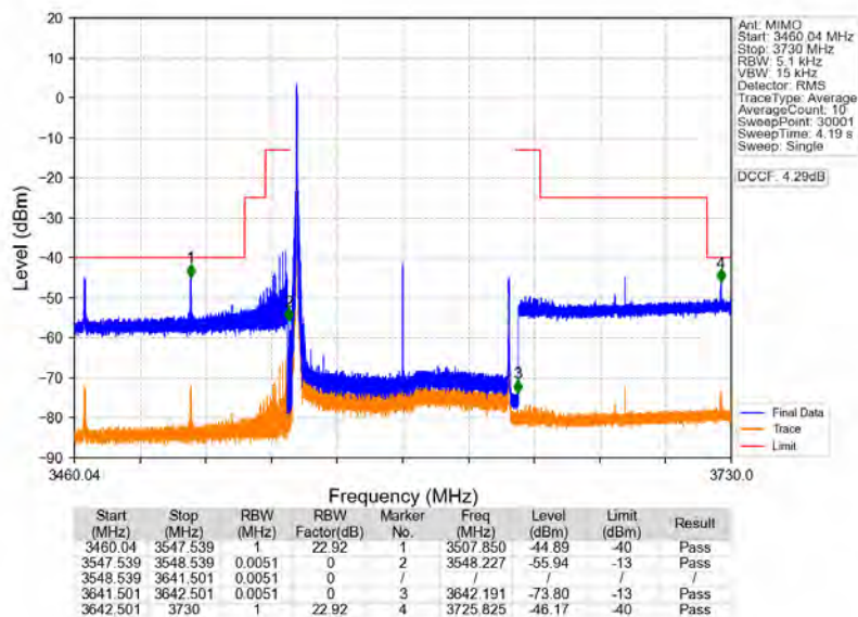
n78d_30kHz_MIMO_NTNV_90MHz_CP-OFDM_QPSK_3595.02MHz_Inner_1RB_Left
