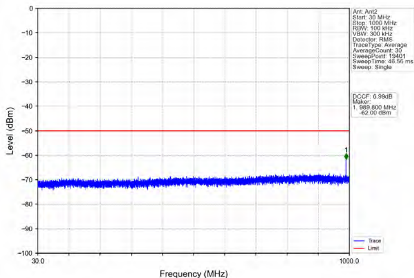
n78d_30kHz_MIMO_NTNV_100MHz_CP-OFDM_QPSK_3600MHz_Edge_1RB_Left
