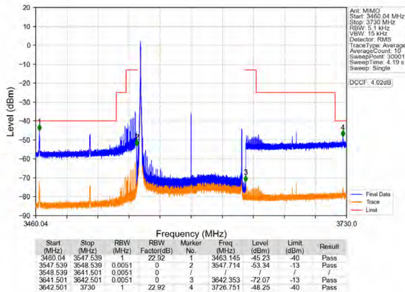
n78d_30kHz_MIMO_NTNV_90MHz_CP-OFDM_QPSK_3595.02MHz_Edge_1RB_Left
