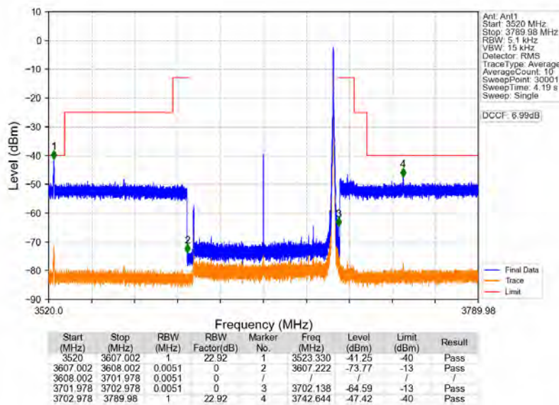
n78d_30kHz_MIMO_NTNV_90MHz_CP-OFDM_QPSK_3654.99MHz_Edge_1RB_Right
