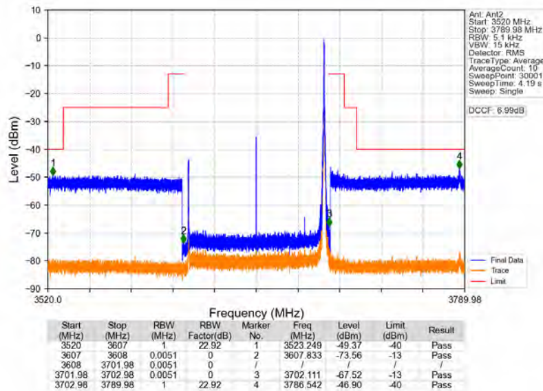
n78d_30kHz_MIMO_NTNV_90MHz_CP-OFDM_QPSK_3654.99MHz_Edge_1RB_Right
