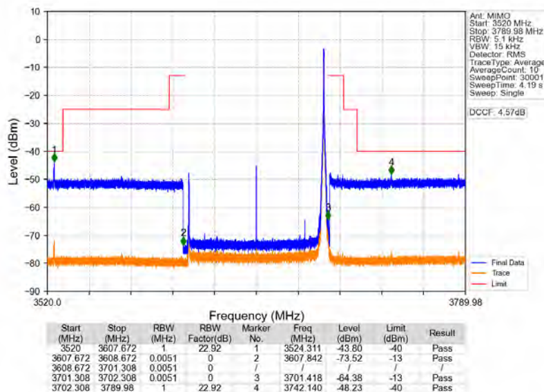
n78d_30kHz_MIMO_NTNV_90MHz_CP-OFDM_QPSK_3654.99MHz_Inner_1RB_Right
