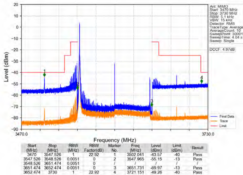
n78d_30kHz_MIMO_NTNV_100MHz_CP-OFDM_QPSK_3600MHz_Edge_1RB_Left
