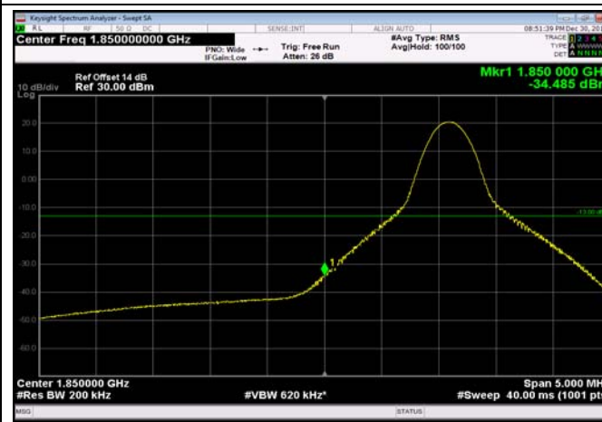
LowRange_FDD02_20MHz_1860_OneRB _low_QPSK
