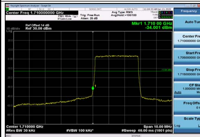
LowRange_FDD04_5MHz_1712.5_OneRB _low_QPSK
