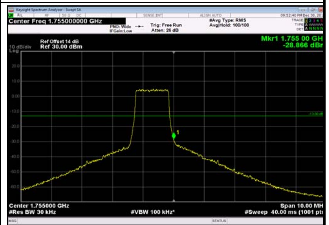
HighRange_FDD04_1.4MHz_1754.3 _fullRB_High_Q16
