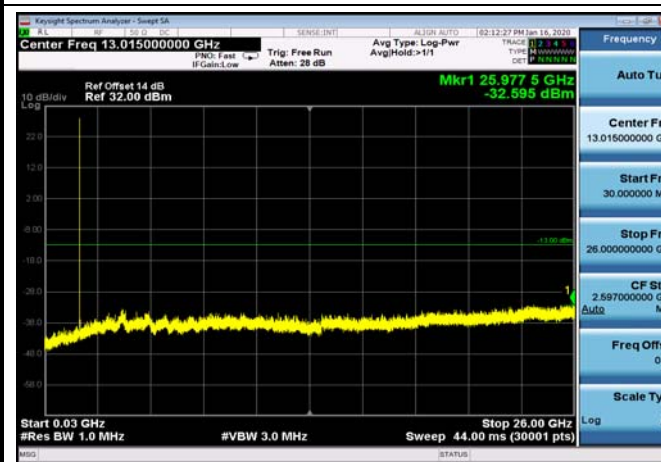
FDD66_MidRange_15MHz_30MHz~26GHz
