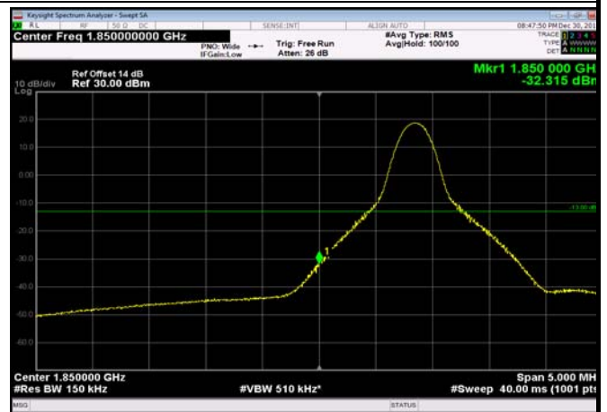
LowRange_FDD02_15MHz_1857.5_fullIRB _Low_Q16
