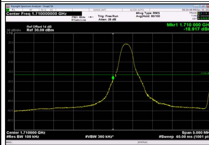
LowRange_FDD04_5MHz_1712.5_OneRB _low_QPSK
