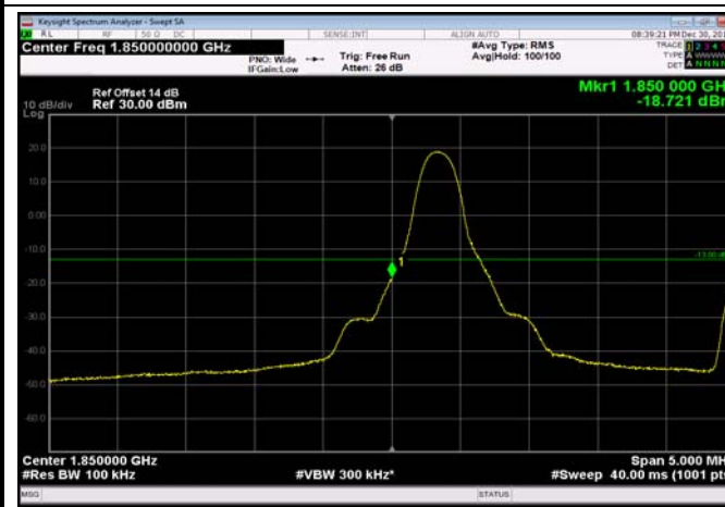
LowRange_FDD02_5MHz_1852.5_OneRB _low_QPSK
