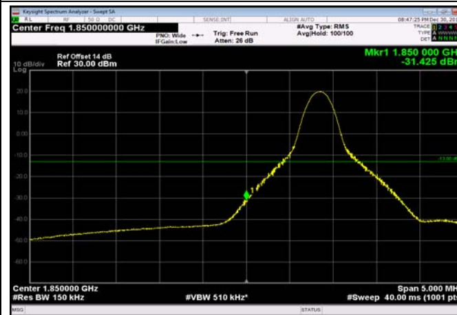
LowRange_FDD02_15MHz_1857.5_fullIRB _Low_QPSK
