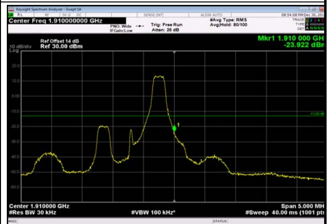
HighRange_FDD02_1.4MHz_1909.3 _fullRB_High_Q16
