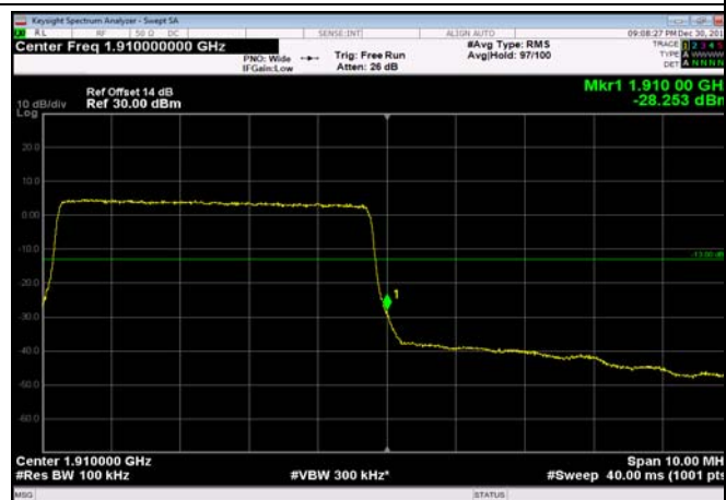
HighRange_FDD02_10MHz_1905_OneRB high Q16
