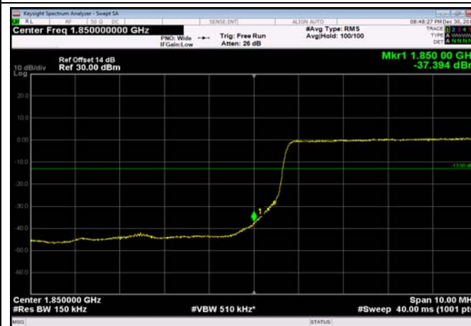
LowRange_FDD02_20MHz_1860_OneRB _low_QPSK
