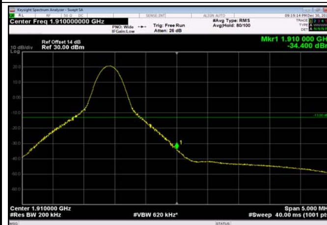
HighRange_FDD02_20MHz_1900_OneRB _high_QPSK
