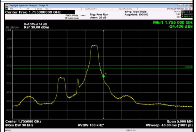
HighRange_FDD04_1.4MHz_1754.3 _fullRB_High_Q16
