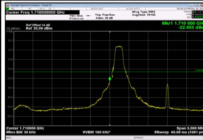
LowRange_FDD04_3MHz_1711.5_fullRB _Low_QPSK
