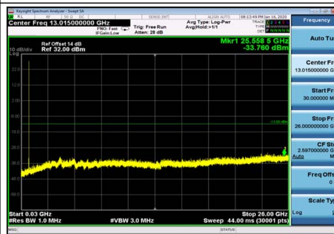
FDD14_LowRange_5MHz_30MHz~26GHz
