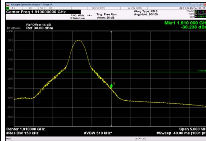
HighRange_FDD02_15MHz_1902.5_fullRB _High_QPSK
