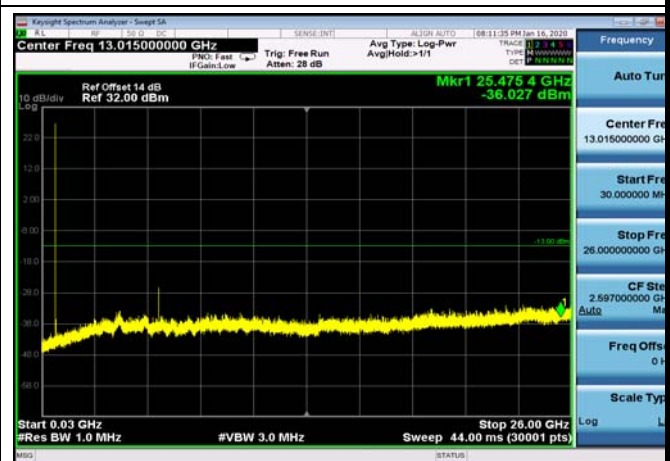
FDD12_LowRange_5MHz_30MHz~26GHz
