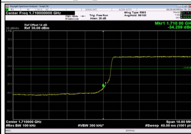
LowRange_FDD04_10MHz_1715_fullRB _Low_QPSK
