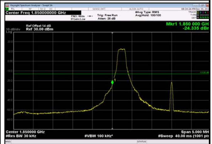
LowRange_FDD02_3MHz_1851.5_fullIRB _Low_Q16
