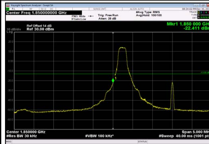
LowRange_FDD02_3MHz_1851.5_fullIRB _Low_QPSK
