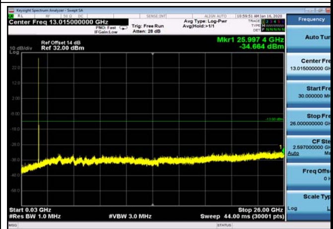
FDD66_MidRange_3MHz_30MHz~26GHz
