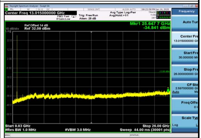
FDD14_HighRange_5MHz_30MHz~26GHz
