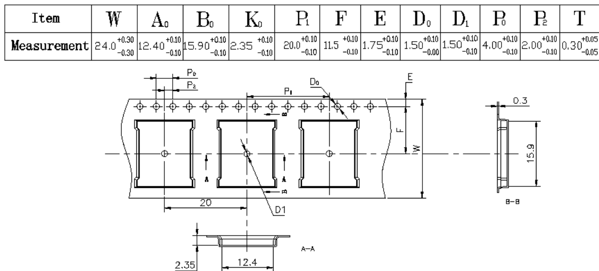
Figure 20. CYBT-343052-02 Tape Dimensions
