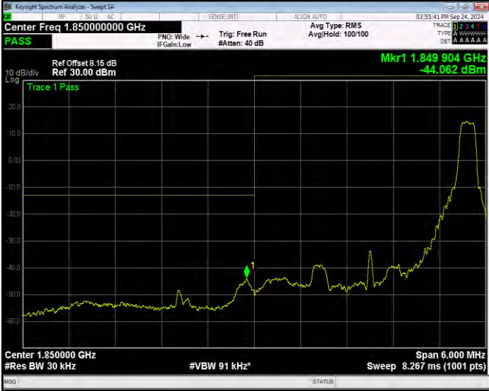
Band25 QPSK BW=3MHz Channel=26055 RB Size=15 Position=#0 Extended
