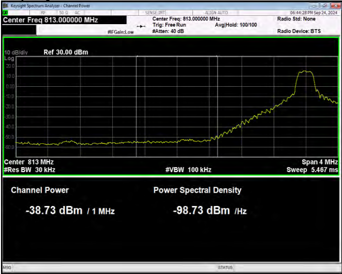
Band26(814-824) 16QAM BW=10MHz Channel=26740 RB Size=1 Position=#0 Normal
