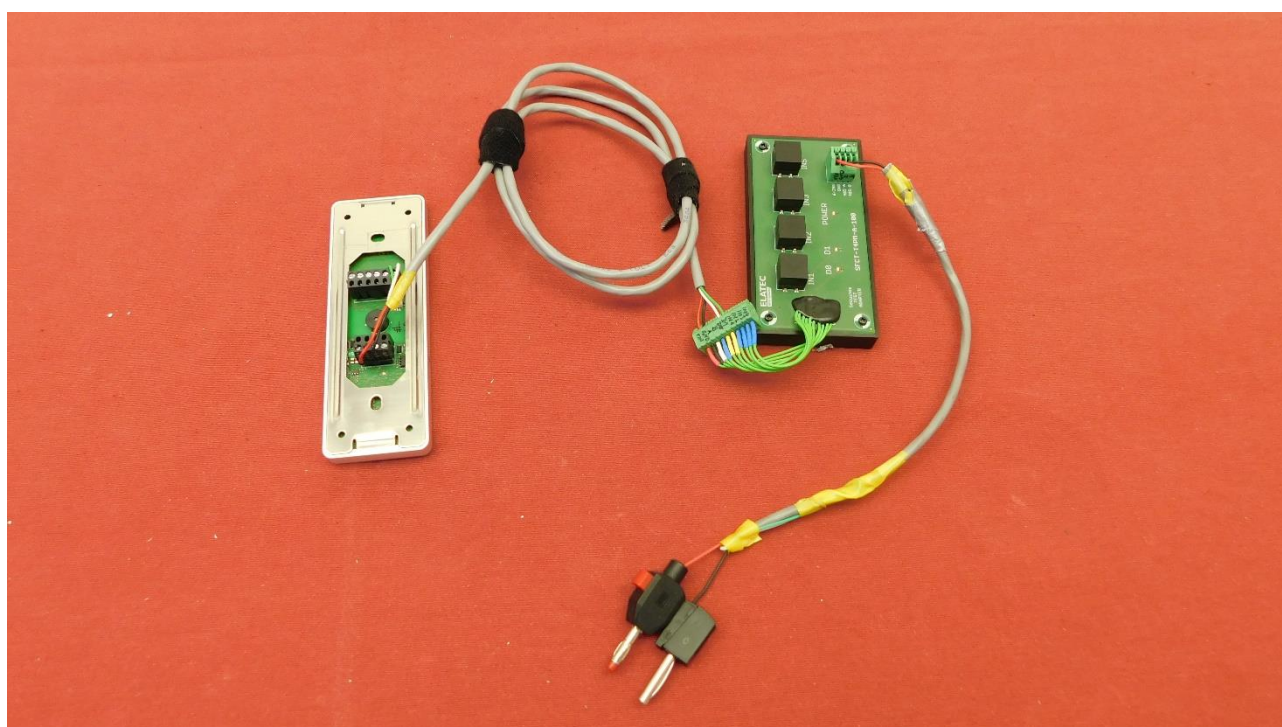
Picture 14: EUT connected with Wiegand adapter rear view
