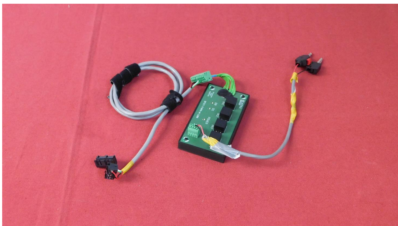
Picture 12: Wiegand adapter
