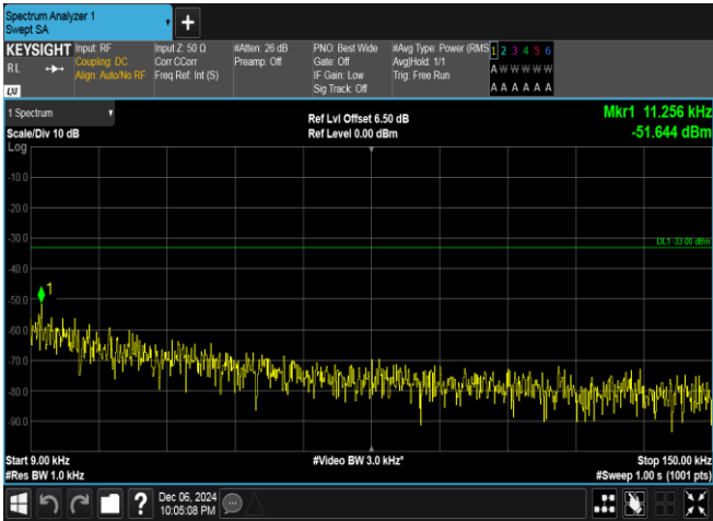
Band5-4182-3-0.009~0.15MHz-PASS
