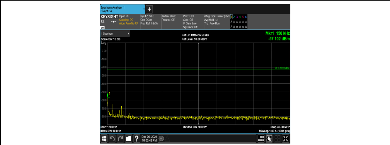
Band5-4233-2-0.15~30MHz-PASS
