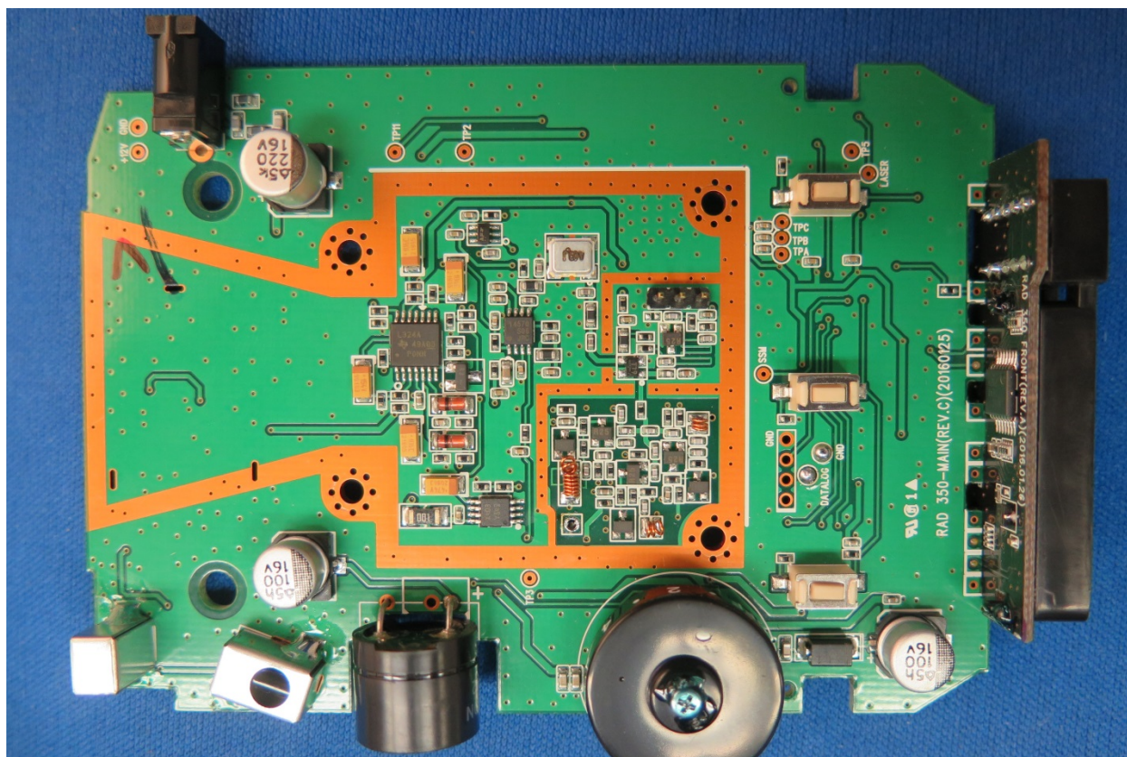
TOP PCB WITH HORN REMOVED
