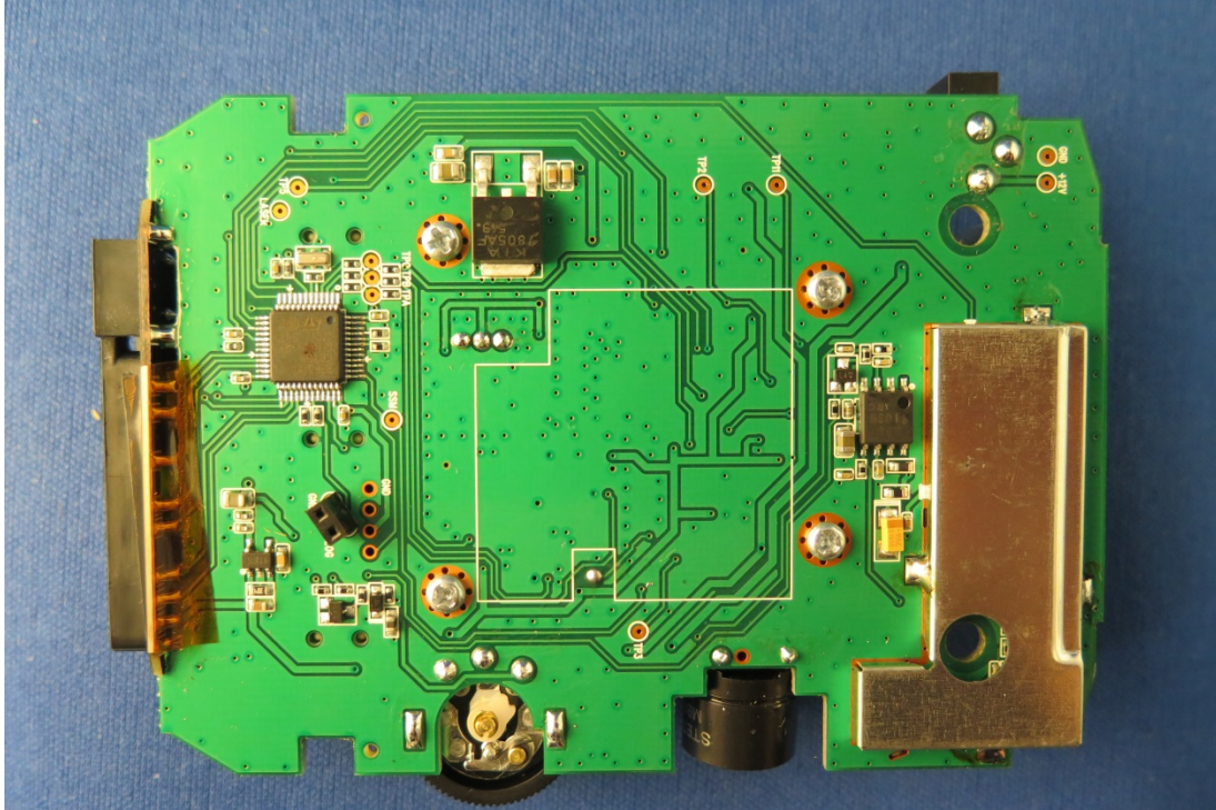
BOTTOM PCB WITH LASER SHIELD
