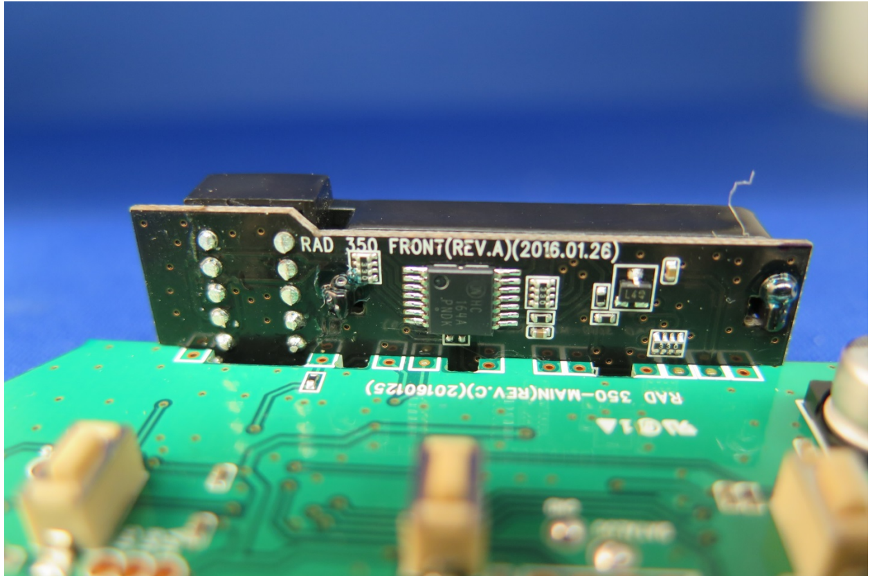
PCB BEHIND DISPLAY
