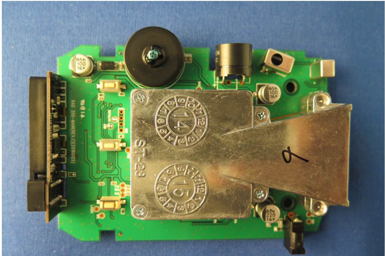
TOP PCB WITH HORN
