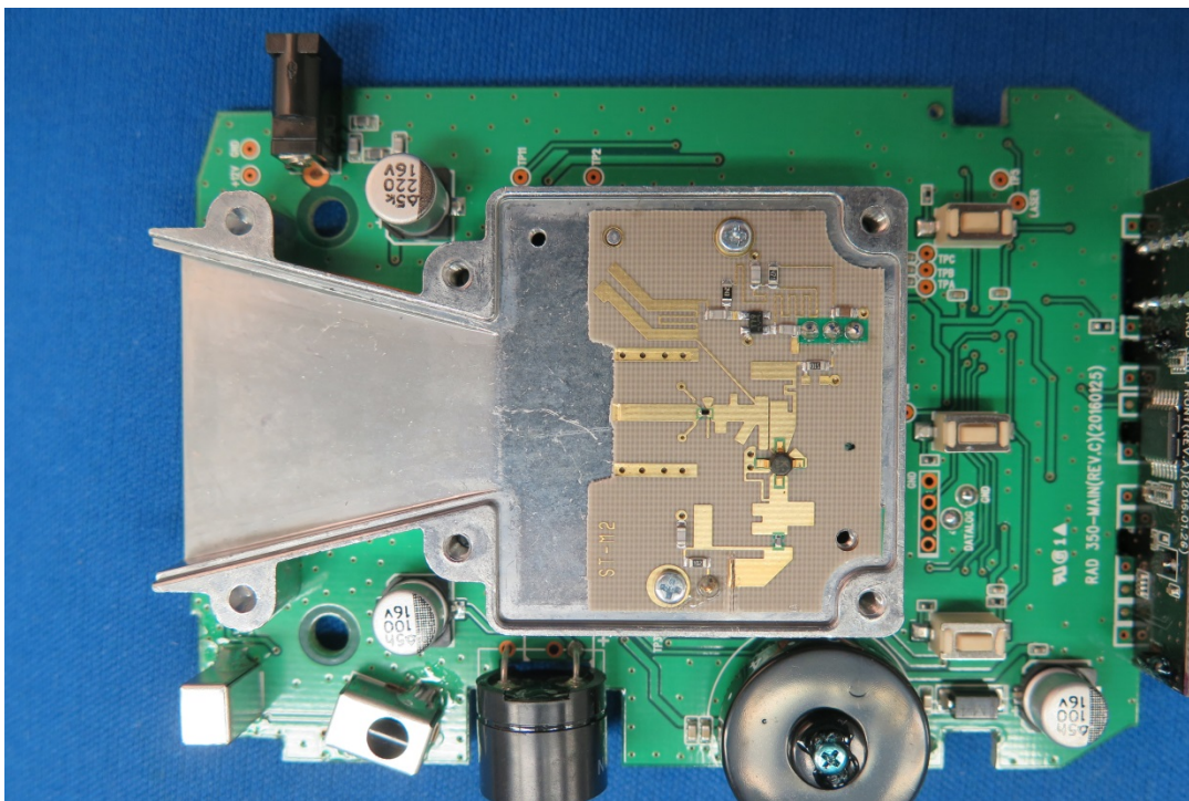
TOP PCB WITH TOP OF HORN REMOVED
