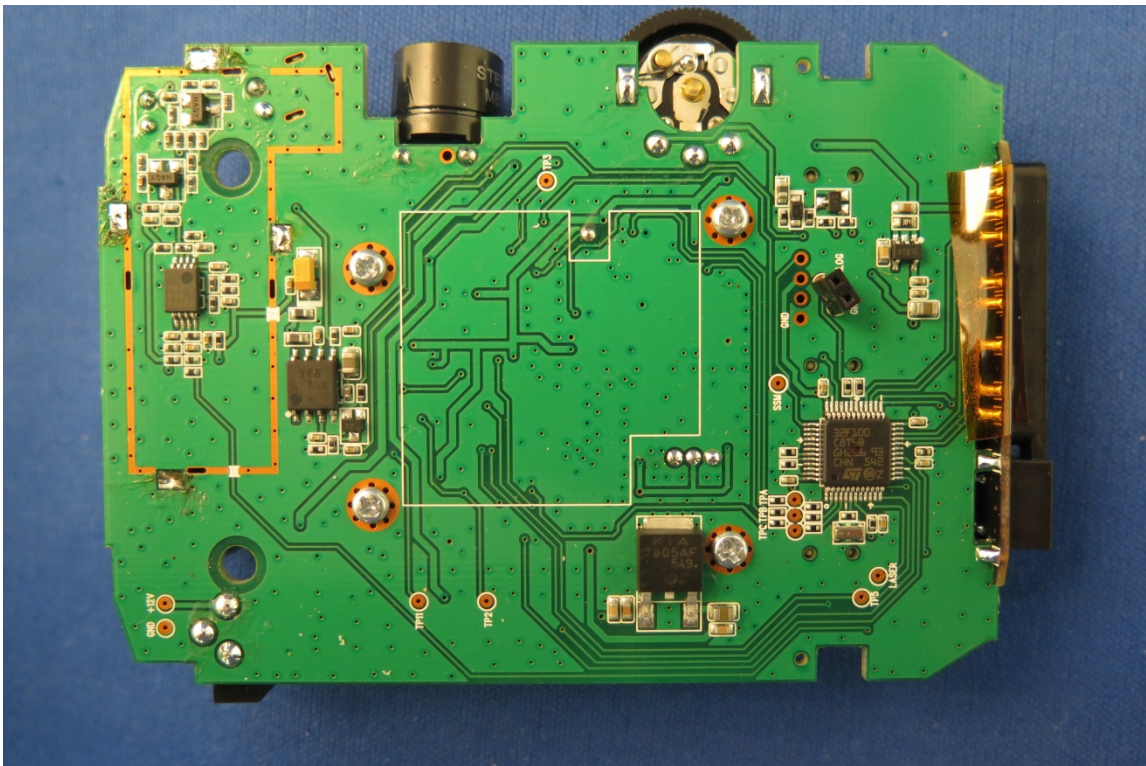
BOTTOM PCB WITHOUT LASER SHIELD
