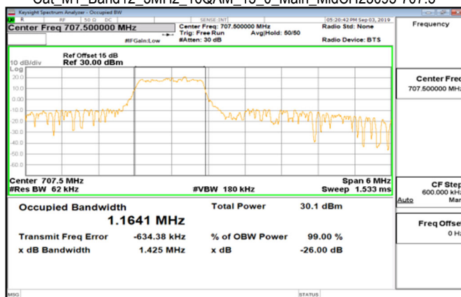
Cat_M1_Band12_3MHz_16QAM_15_0_Main_MidCH23095-707.5
