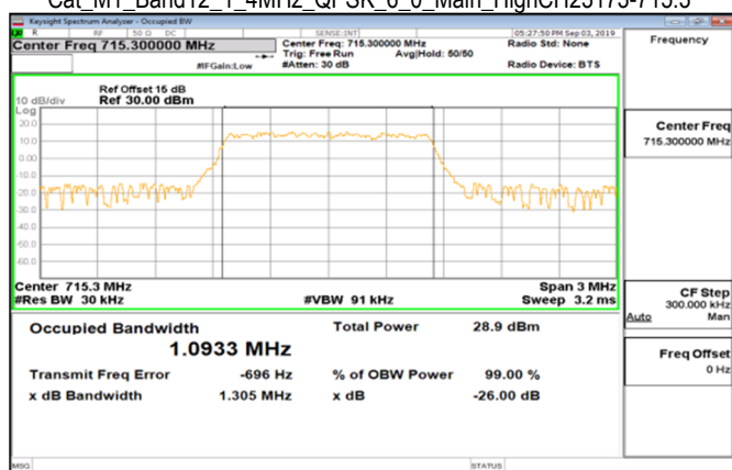
Cat_M1_Band12_1_4MHz_QPSK_6_0_Main_HighCH23173-715.3
