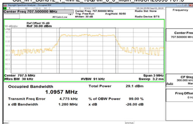
Cat_M1_Band12_1_4MHz_16QAM_6_0_Main_MidCH23095-707.5
