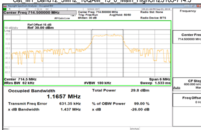
Cat_M1_Band12_3MHz_16QAM_15_0_Main_HighCH23165-714.5
