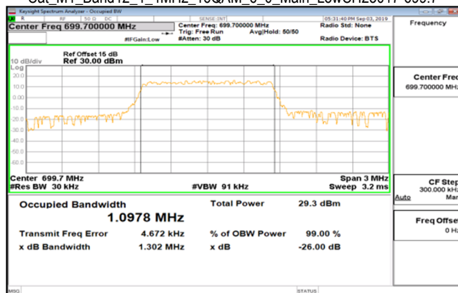
Cat_M1_Band12_1_4MHz_16QAM_6_0_Main_LowCH23017-699.7
