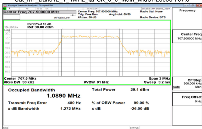
Cat_M1_Band12_1_4MHz_QPSK_6_0_Main_MidCH23095-707.5
