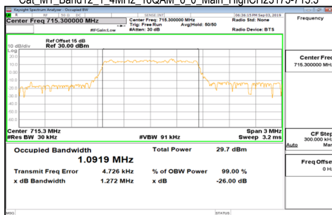
Cat_M1_Band12_1_4MHz_16QAM_6_0_Main_HighCH23173-715.3
