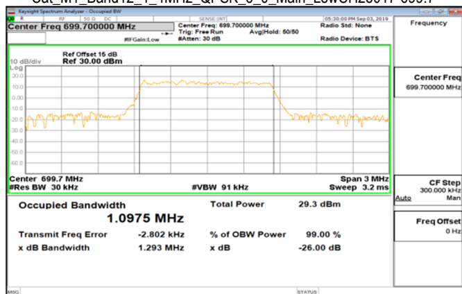
Cat_M1_Band12_1_4MHz_QPSK_6_0_Main_LowCH23017-699.7
