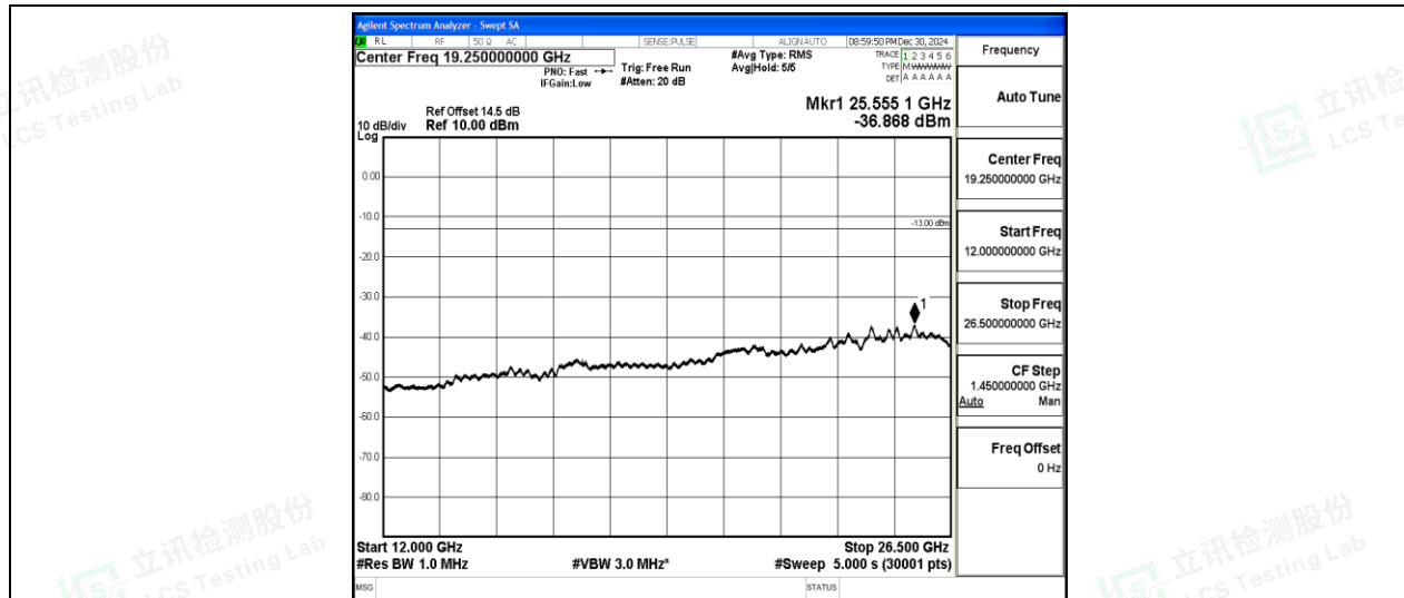
Band2-15MHz-QPSK-18900-1-0-Low-12000-26500--36.87-PASS
