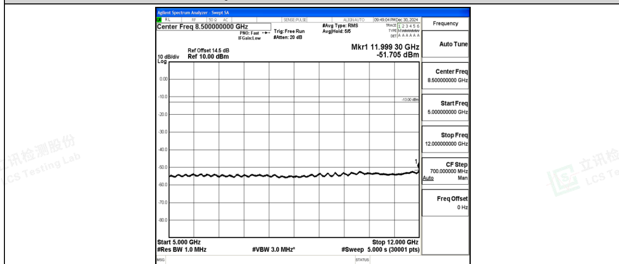
Band2-20MHz-QPSK-18700-1-0-Low-5000-12000--51.71-PASS
