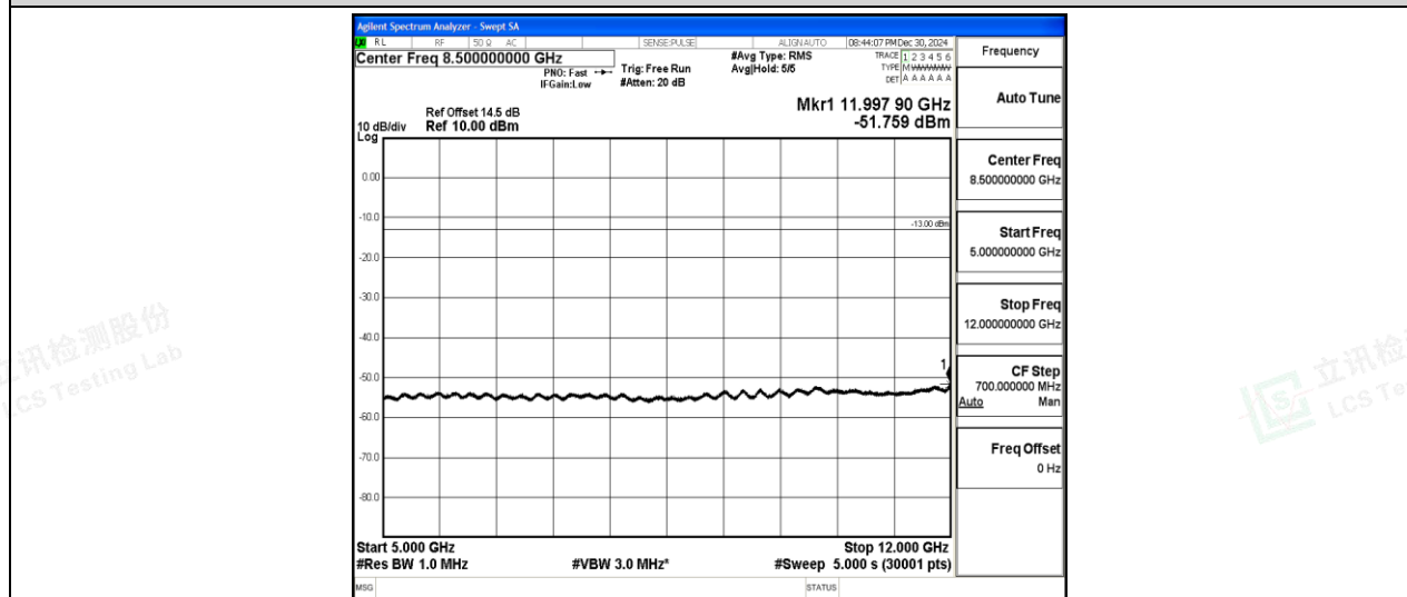
Band2-15MHz-16QAM-18675-1-0-Low-5000-12000--51.76-PASS
