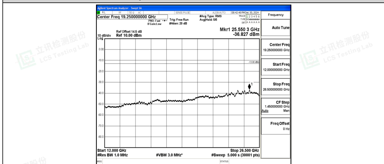
Band2-15MHz-QPSK-18675-1-0-Low-12000-26500--36.83-PASS
