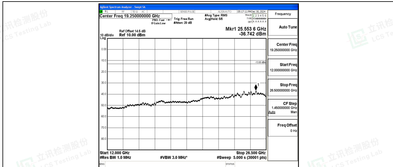
Band2-5MHz-16QAM-18900-1-0-Low-12000-26500--36.74-PASS
