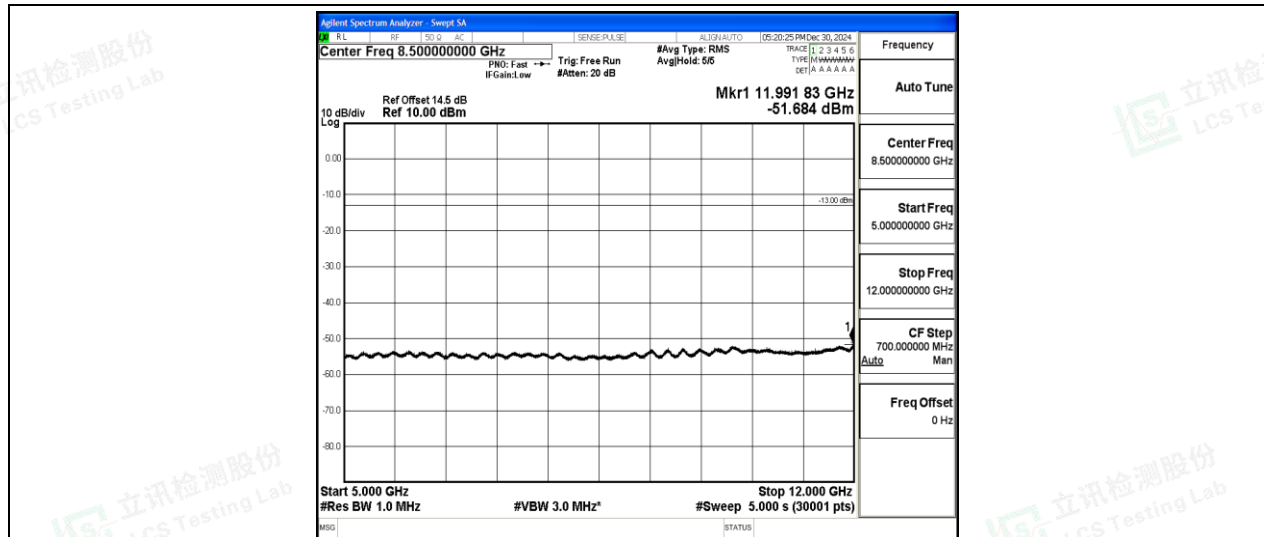
Band2-5MHz-16QAM-19175-1-0-High-5000-12000--51.68-PASS
