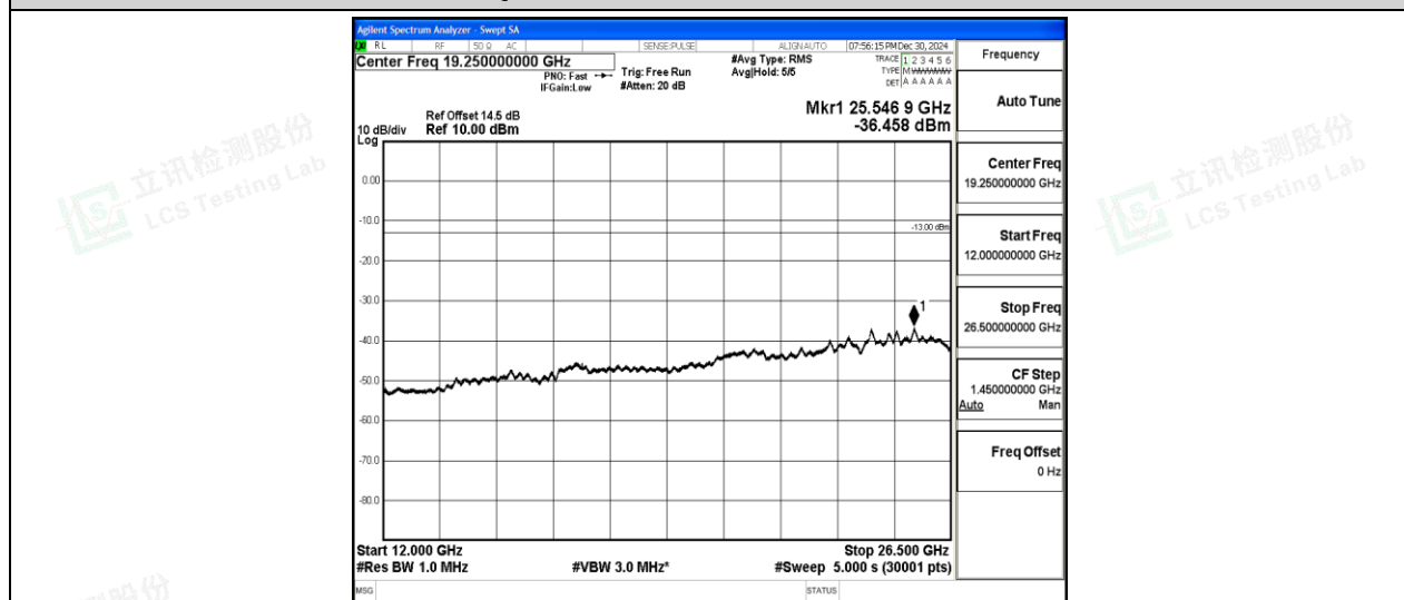
Band2-10MHz-QPSK-18650-1-0-Low-12000-26500--36.46-PASS
