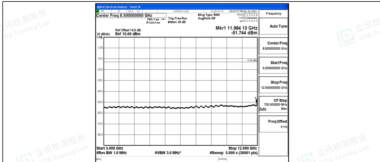
Band2-15MHz-16QAM-19125-1-0-High-5000-12000--51.74-PASS
