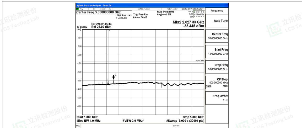
Band2-15MHz-16QAM-18675-1-0-Low-1000-5000--33.45-PASS
