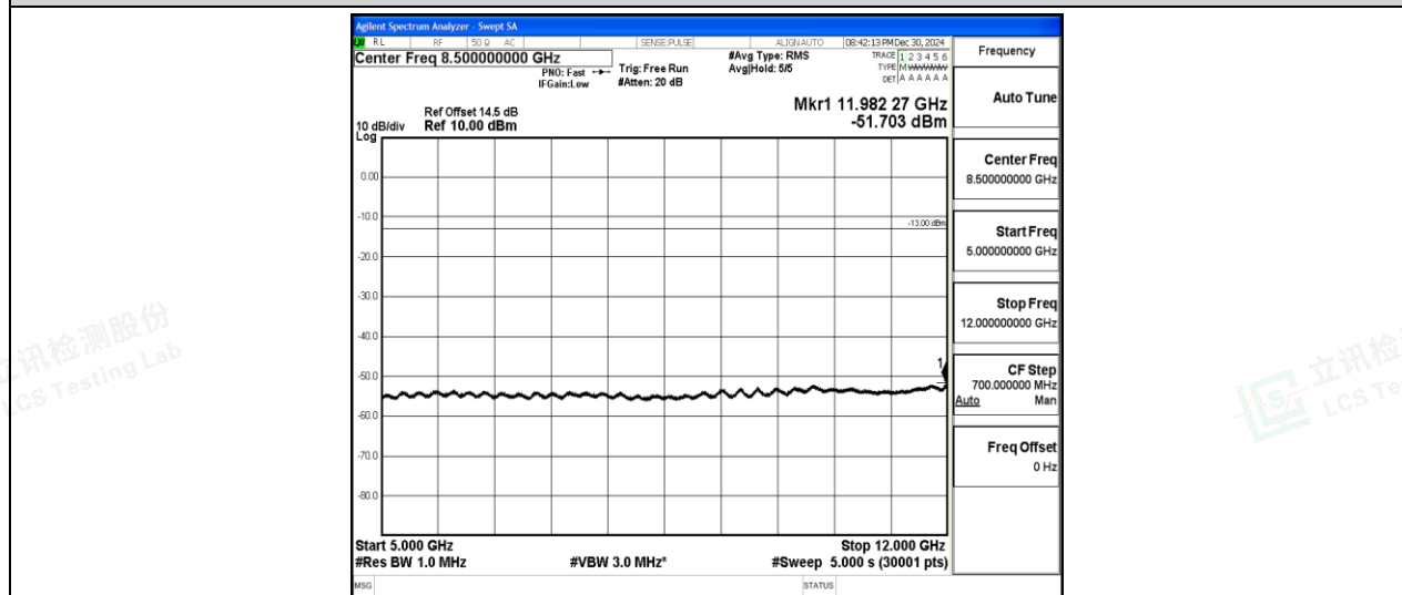
Band2-15MHz-QPSK-18675-1-0-Low-5000-12000--51.7-PASS
