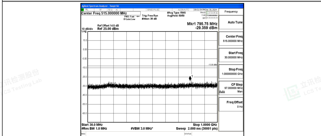
Band2-15MHz-QPSK-19125-1-0-High-30-1000--29.36-PASS
