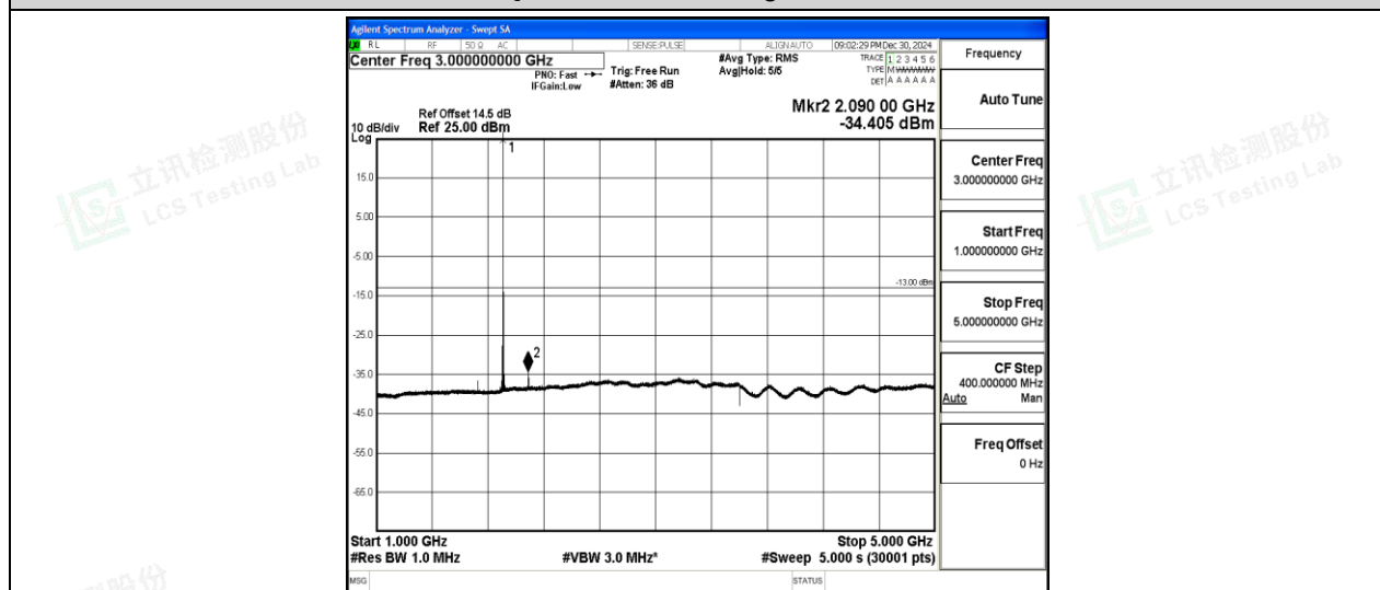
Band2-15MHz-QPSK-19125-1-0-High-1000-5000--34.41-PASS
