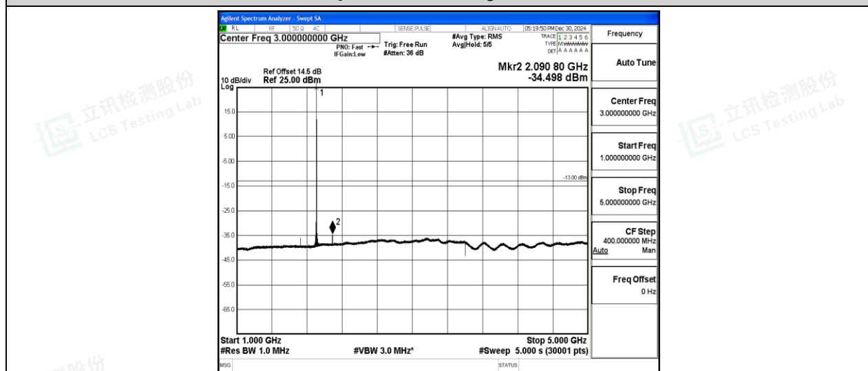
Band2-5MHz-16QAM-19175-1-0-High-1000-5000--34.5-PASS
