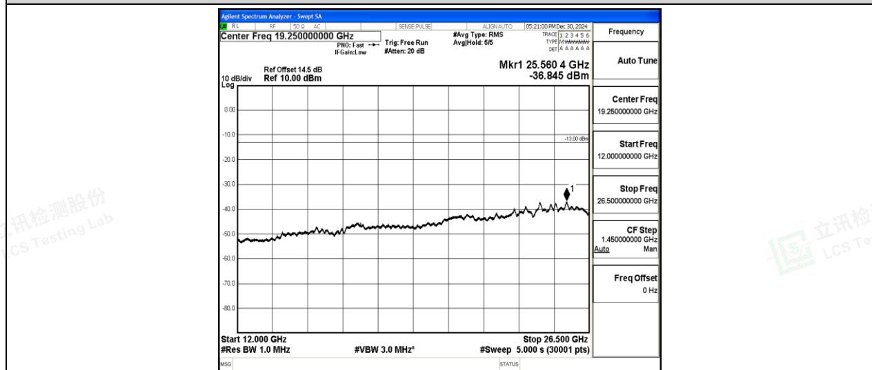
Band2-5MHz-16QAM-19175-1-0-High-12000-26500--36.85-PASS
