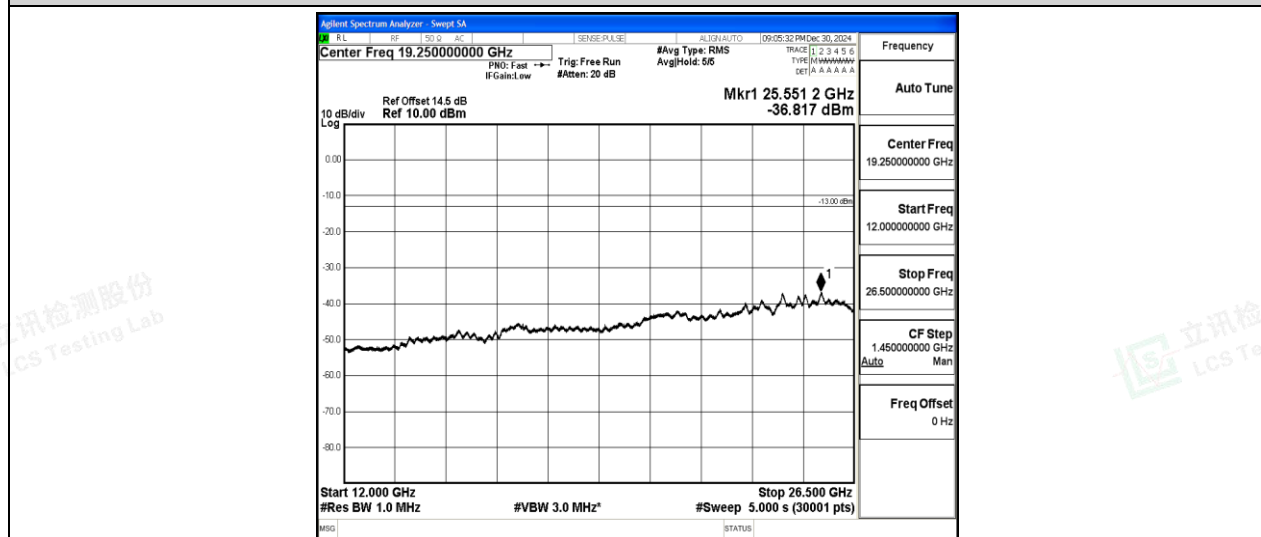
Band2-15MHz-16QAM-19125-1-0-High-12000-26500--36.82-PASS
