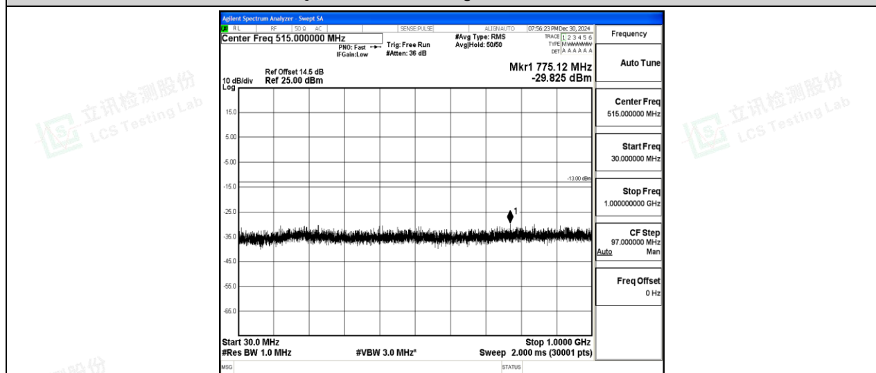
Band2-10MHz-16QAM-18650-1-0-Low-30-1000--29.83-PASS
