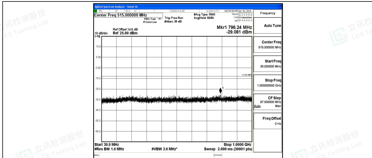
Band2-15MHz-16QAM-18900-1-0-Low-30-1000--29.08-PASS
