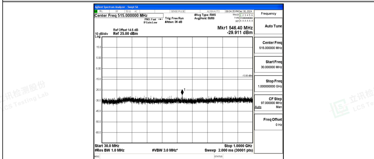
Band2-10MHz-16QAM-19150-1-0-High-30-1000--29.91-PASS
