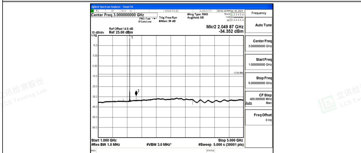
Band2-20MHz-QPSK-18900-1-0-Low-1000-5000--34.35-PASS
