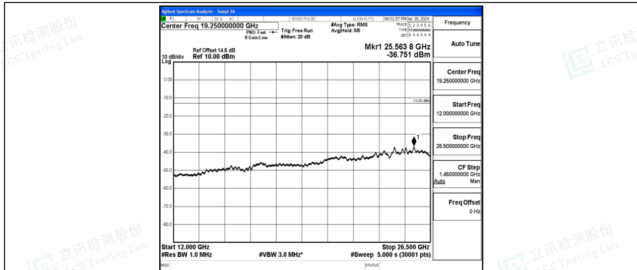
Band2-10MHz-16QAM-18900-1-0-Low-12000-26500--36.75-PASS
