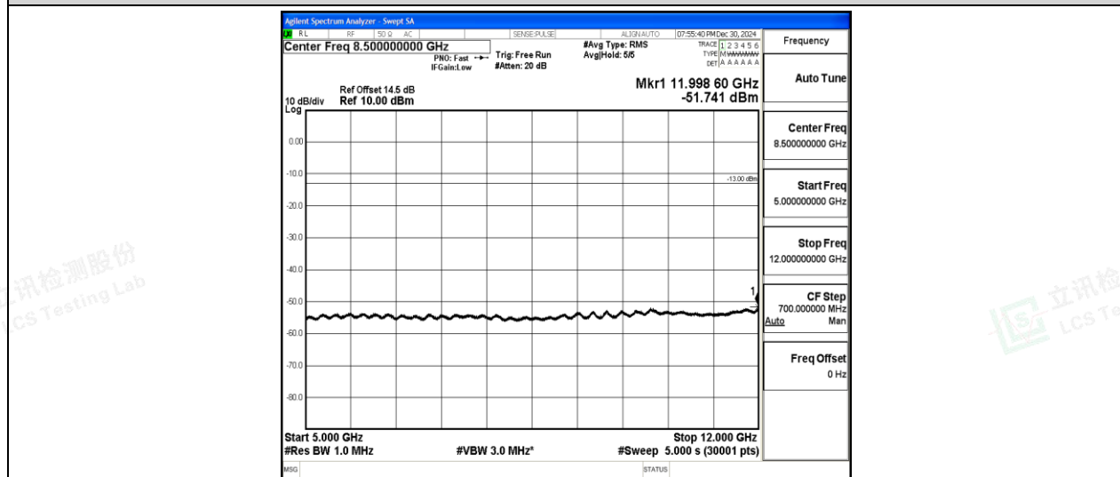
Band2-10MHz-QPSK-18650-1-0-Low-5000-12000--51.74-PASS
