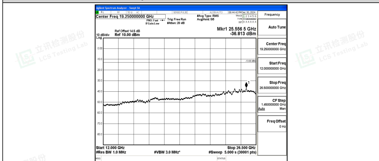
Band2-15MHz-16QAM-18675-1-0-Low-12000-26500--36.81-PASS
