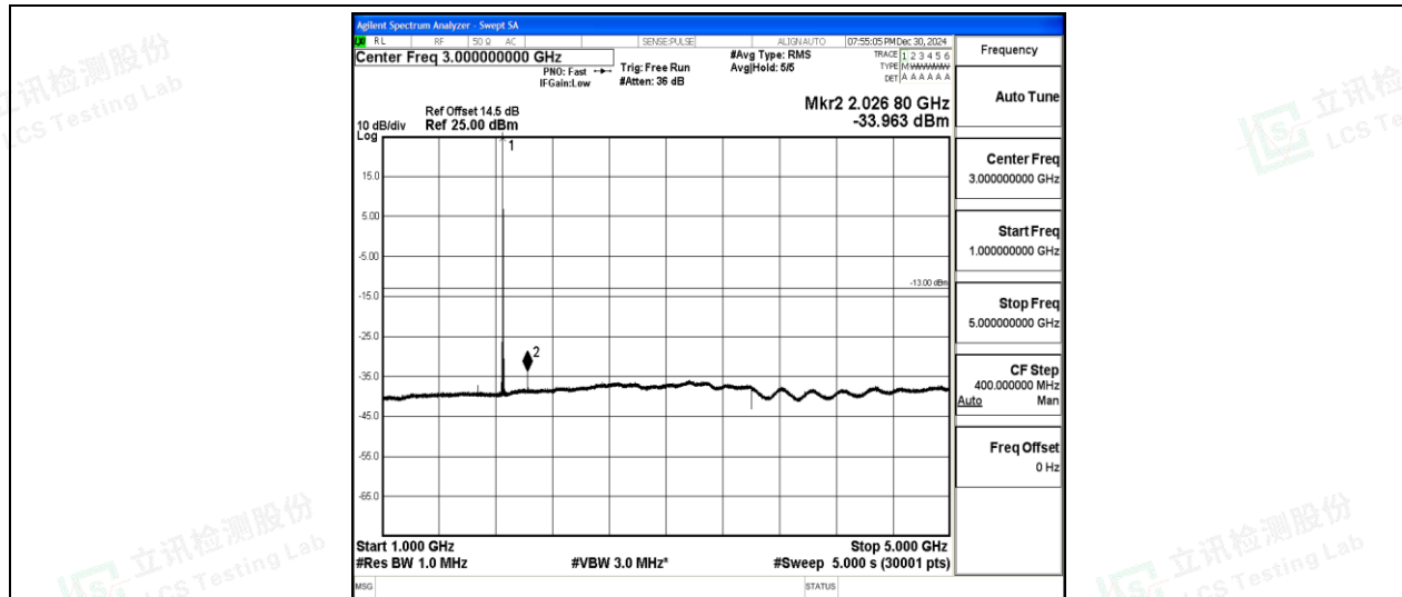
Band2-10MHz-QPSK-18650-1-0-Low-1000-5000--33.96-PASS
