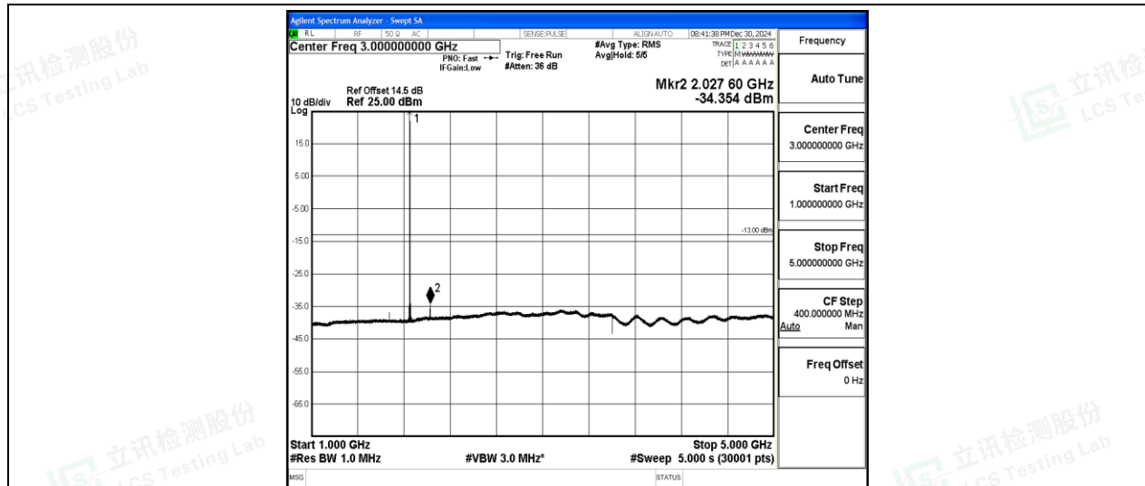
Band2-15MHz-QPSK-18675-1-0-Low-1000-5000--34.35-PASS
