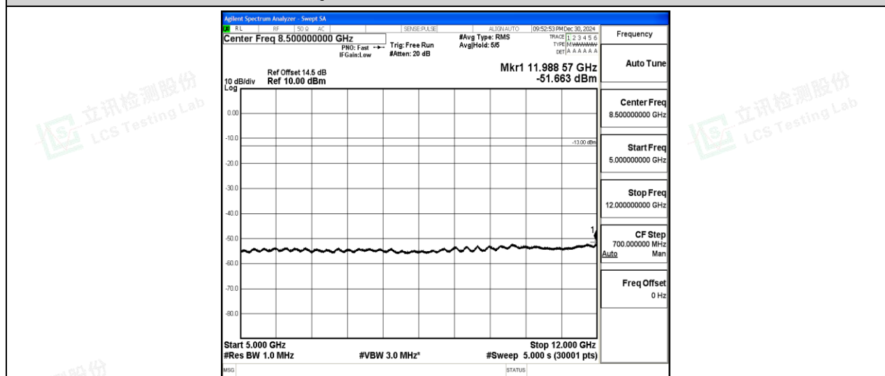
Band2-20MHz-QPSK-18900-1-0-Low-5000-12000--51.66-PASS
