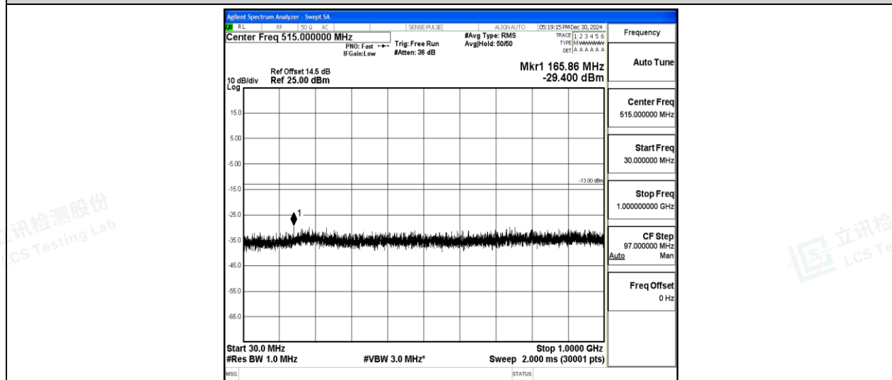
Band2-5MHz-16QAM-19175-1-0-High-30-1000--29.4-PASS
