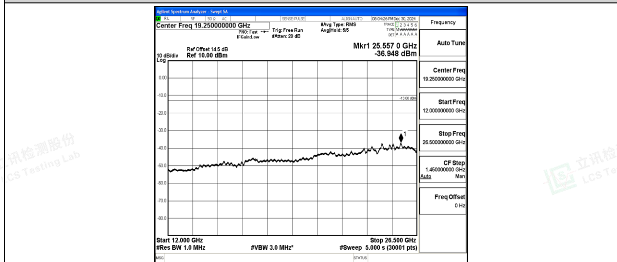
Band2-10MHz-QPSK-19150-1-0-High-12000-26500--36.95-PASS
