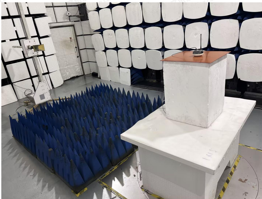
Fig.2 (Above 1GHz)
