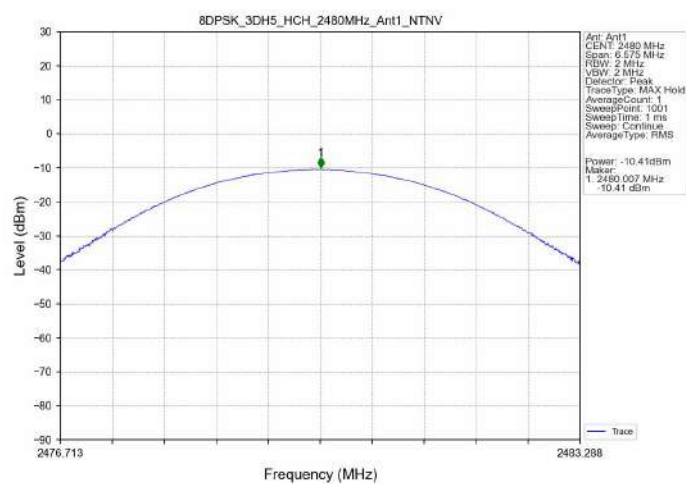
8DPSK_3DH5_HCH_2480MHz_Ant1_NTNV
