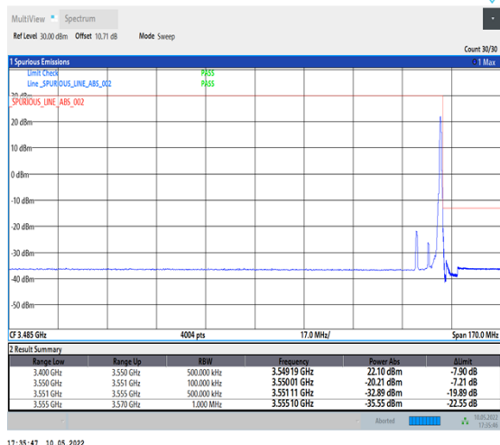
1-N78-3450-3550-PC2-30-10-H-5-CP-QPSK-Edge_1RB_Right-1@23-Ant1-PASS-see graph
