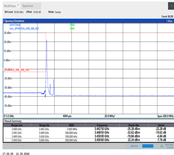
1-N78-3450-3550-PC2-30-10-L-4-CP-QPSK-Edge_1RB_Left-1@0-Ant1-PASS-see graph
