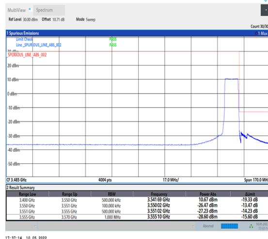
1-N78-3450-3550-PC2-30-10-H-6-CP-QPSK-Outer_Full-24@0-Ant1-PASS-see graph
