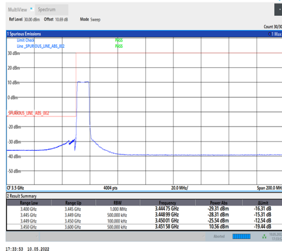
1-N78-3450-3550-PC2-30-10-L-6-CP-QPSK-Outer_Full-24@0-Ant1-PASS-see graph
