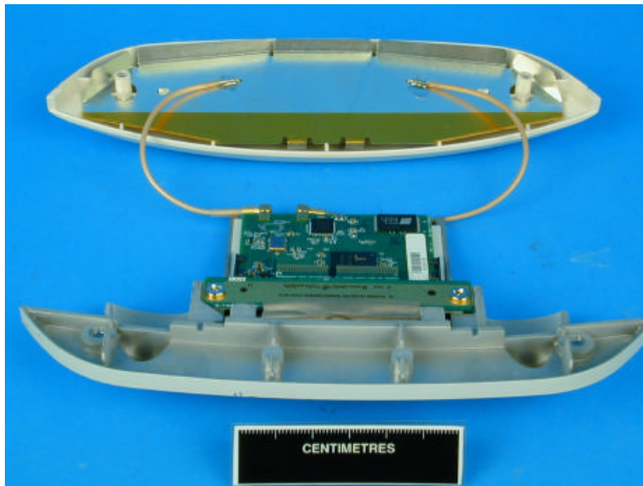
Photo 6; Internal of Integral Antenna
