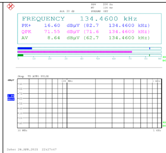
INT1 Antenna
