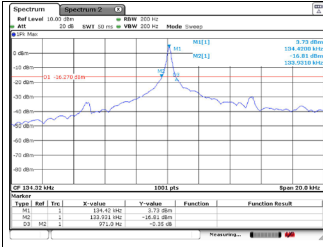
INT2 Antenna
