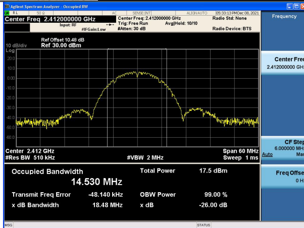
Test Mode:802.11b 2412MHz Chain0
