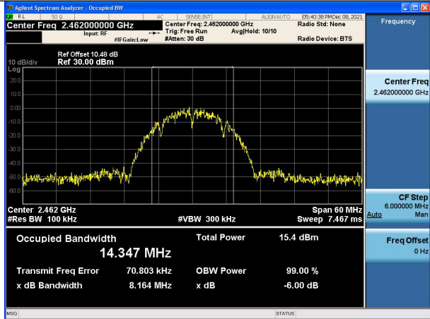
Test Mode:802.11b 2462MHz Chain0
