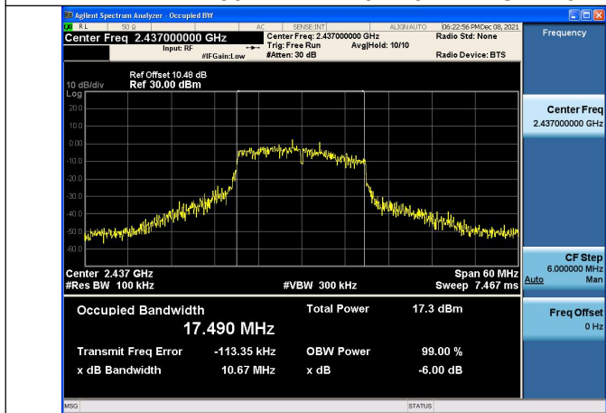
Test Mode:802.11n HT20 2437MHz Chain1
