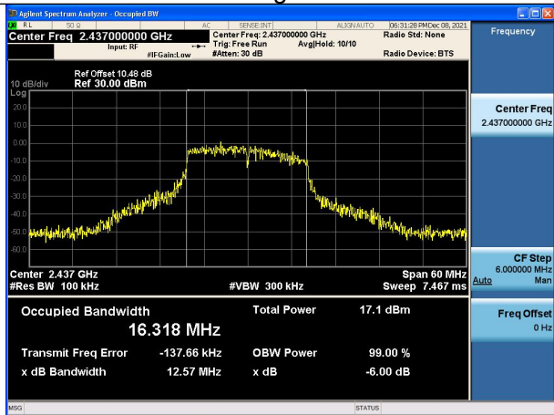
Test Mode:802.11g 2437MHz Chain1
