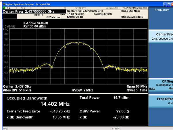
Test Mode:802.11b 2437MHz Chain1
