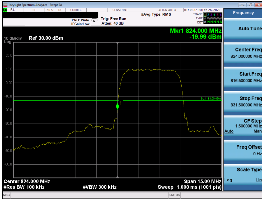
Plot 7-59. Band Edge Plot (Cellular WCDMA Mode - Low Channel)
