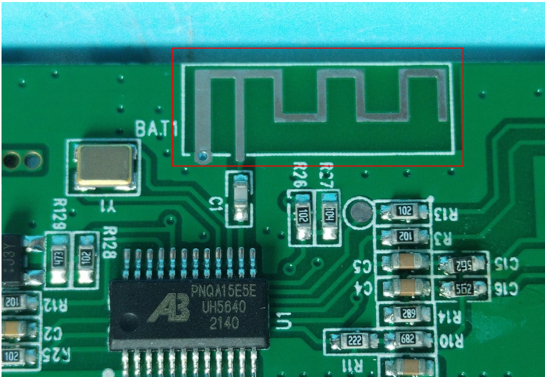
Bluetooth Antenna
