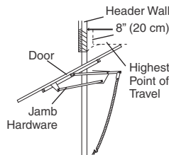
One-piece door without track: jamb hardware
