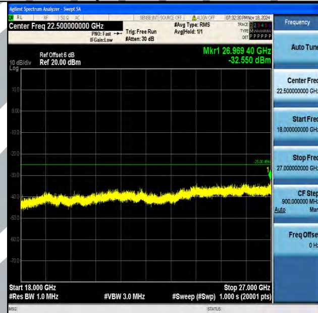
Band7_15MHz_16QAM_20825_1RB#0_18000~27000_18000~27000
