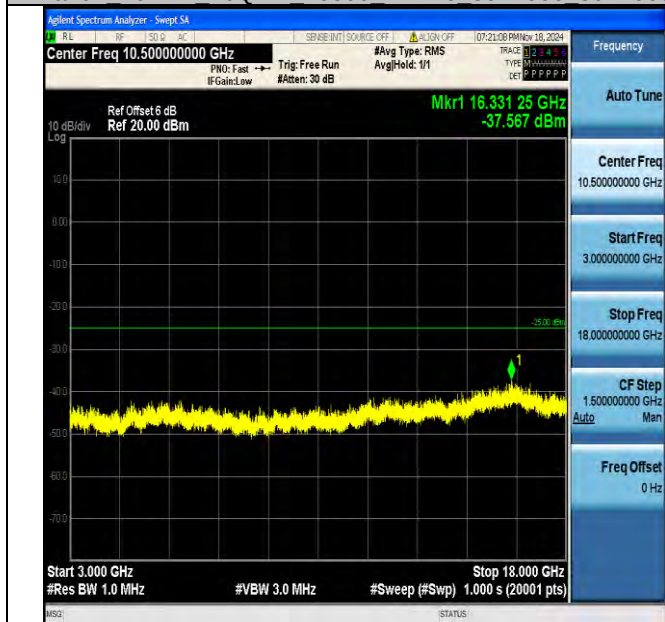
Band7_10MHz_16QAM_20800_1RB#0_3000~18000_3000~18000
