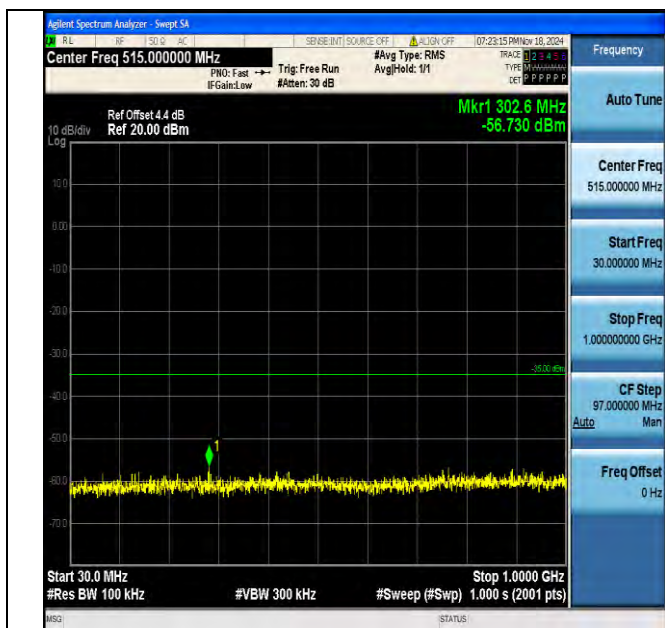
Band7 10MHz 16QAM 21400 1RB#0 30~1000 30~1000
