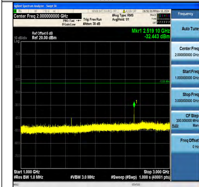
Band5_10MHz_16QAM_20600_1RB#0_1000~3000_1000~3000
