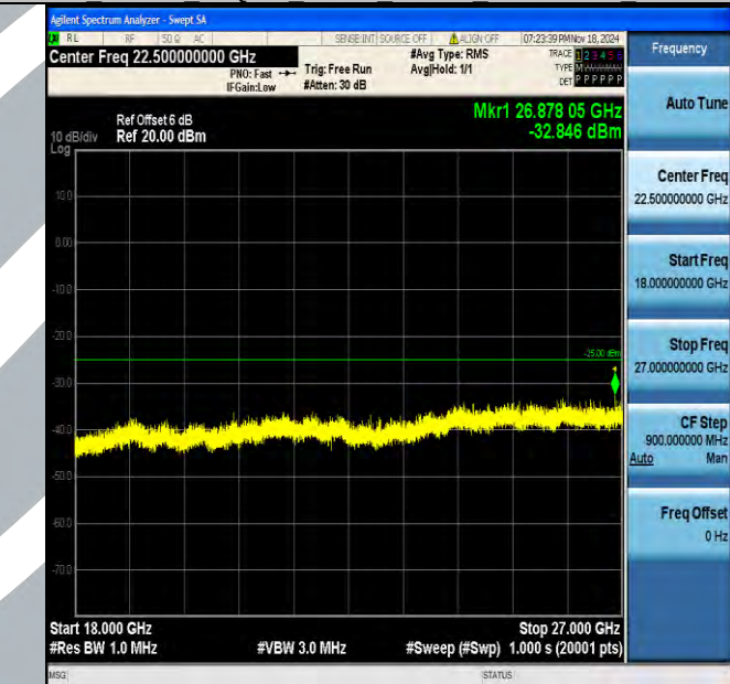
Band7_10MHz_16QAM_21400_1RB#0_18000~27000_18000~27000
