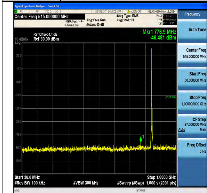
Band5 5MHz QPSK 20625 1RB#0 30~1000 30~1000
