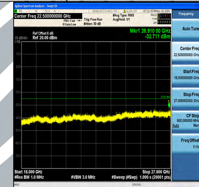
Band7_10MHz_16QAM_20800_1RB#0_18000~27000_18000~27000
