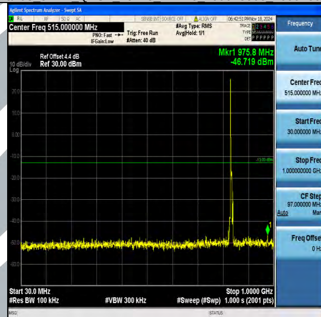
Band5_5MHz_QPSK_20525_1RB#0_30~1000_30~1000
