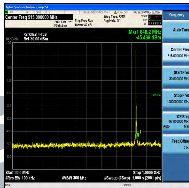
Band5_3MHz_QPSK_20525_1RB#0_30~1000_30~1000
