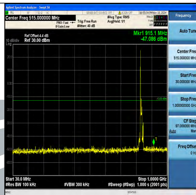
Band5_10MHz_QPSK_20525_1RB#0_30~1000_30~1000
