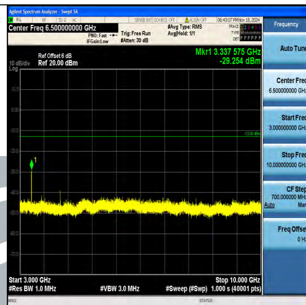
Band5 5MHz QPSK 20525 1RB#0 3000~10000 3000~10000
