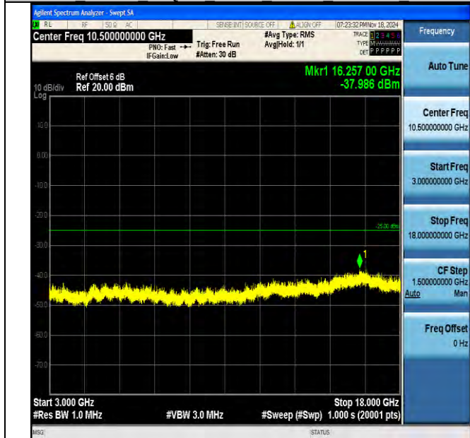
Band7_10MHz_16QAM_21400_1RB#0_3000~18000_3000~18000
