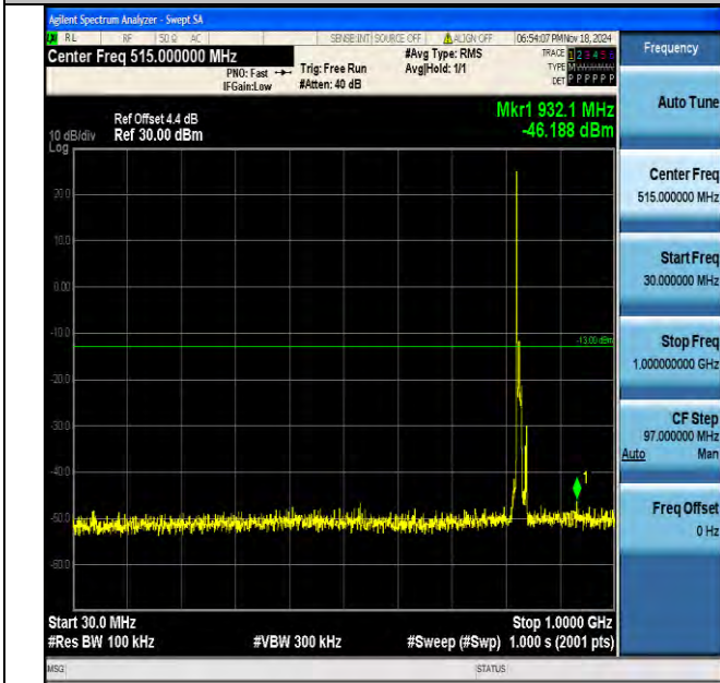
Band5_10MHz_QPSK_20450_1RB#0_30~1000_30~1000
