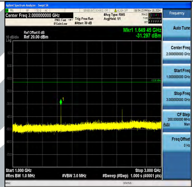
Band5_10MHz_QPSK_20450_1RB#0_1000~3000_1000~3000
