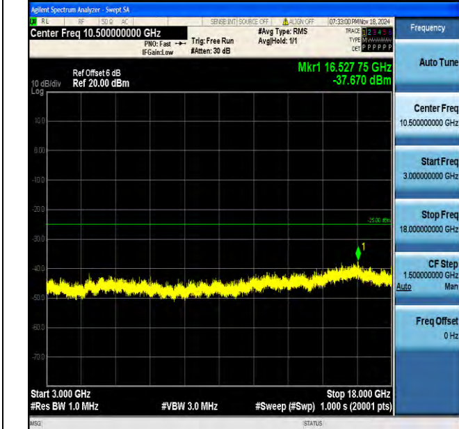
Band7_15MHz_QPSK_21100_1RB#0_3000~18000_3000~18000
