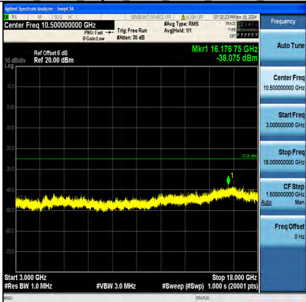
Band7_15MHz_16QAM_20825_1RB#0_3000~18000_3000~18000
