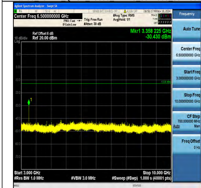
Band5_10MHz_QPSK_20600_1RB#0_3000~10000_3000~10000
