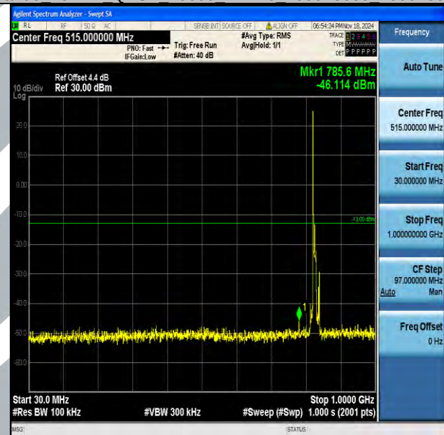
Band5_10MHz_16QAM_20450_1RB#0_30~1000_30~1000
