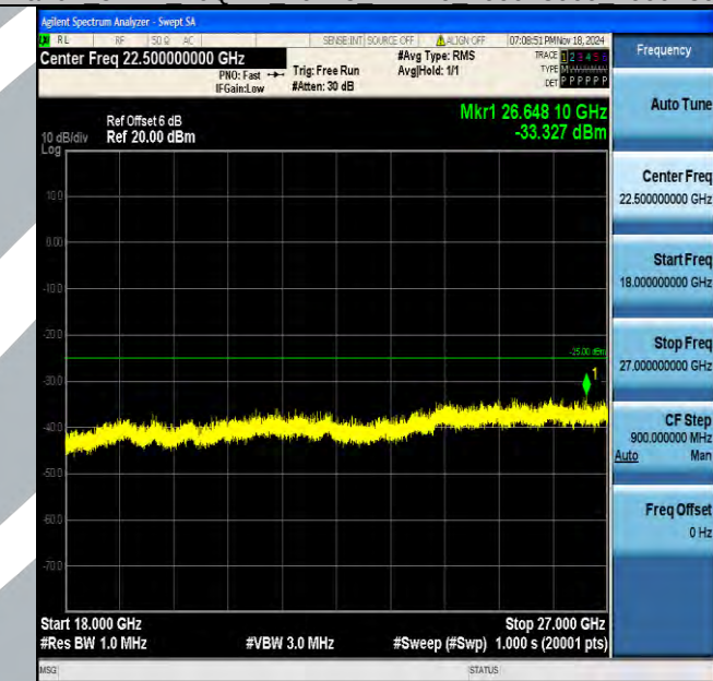
Band7_5MHz_16QAM_20775_1RB#0_18000~27000_18000~27000
