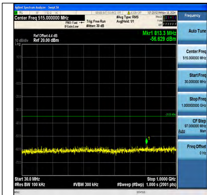
Band7 10MHz 16QAM 20800 1RB#0 30~1000 30~1000
