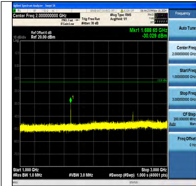
Band5_5MHz_16QAM_20625_1RB#0_1000~3000_1000~3000
