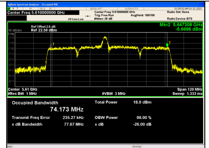
IEEE 802.11ax_Channel 122_80MHz_Antenna 1_RU&Index 26RU17
