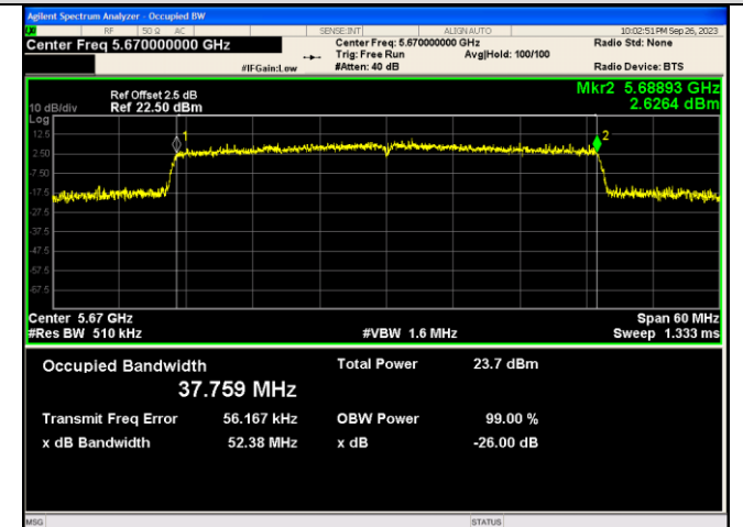
IEEE 802.11ax_Channel 134_40MHz_Antenna 1_RU&Index 484RU65
