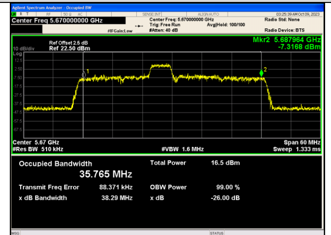
IEEE 802.11ax_Channel 134_40MHz_Antenna 1_RU&Index 52RU40
