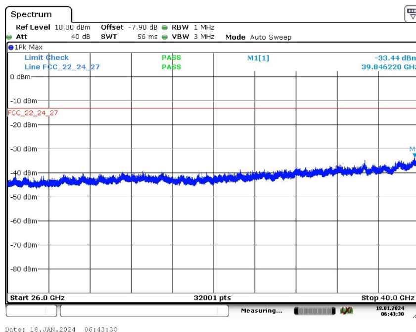
Plot 12: QPSK - Middle channel (26 GHz – 40 GHz), LTE band 42 and WLAN acVHT80-mode
