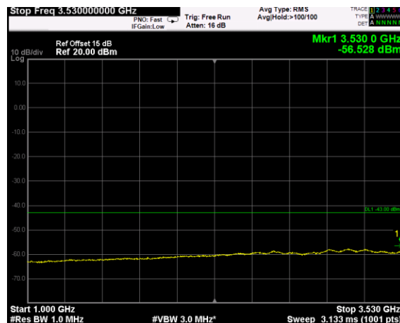
Channel: MIDDLE, Modulation: 64QAM, BW=5MHz, Range: 1GHz - 3530MHz
