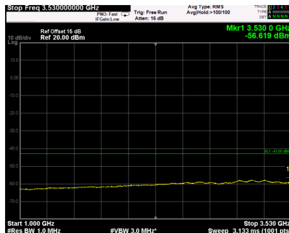
Channel: BOTTOM, Modulation: 16QAM, BW=5MHz, Range: 1GHz - 3530MHz
