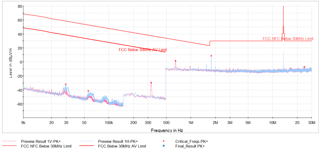
Plot 7-9. Radiated Spurious Emissions 9kHz – 30MHz (Reader A 848kbps, with AC/DC Adapter and Magnetic Charger)
