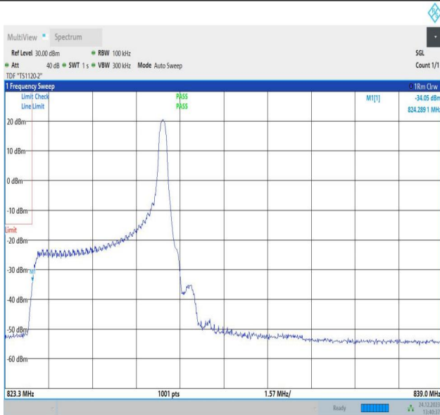
5MHz-10MHz_QPSK@QPSK-QPSK@QPSK_20428-20500_1 RB#0@25RB#0-0RB#0@50RB#0
