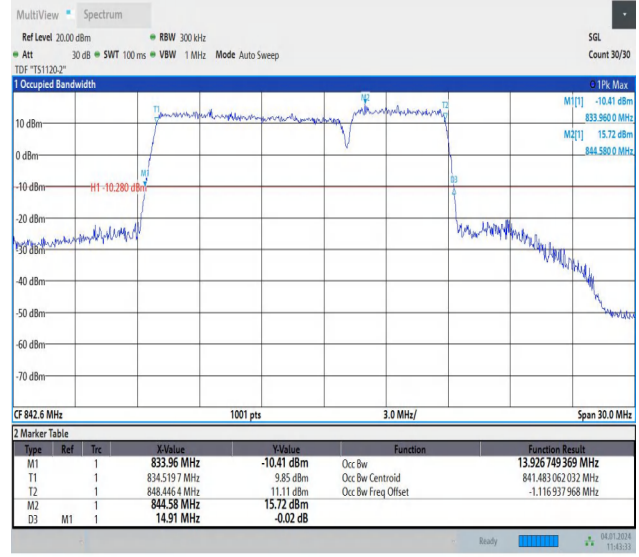
5-5-10MHz-5MHz-64QAM-64QAM-20550-20622-50RB#0-25R B#0-PASS
