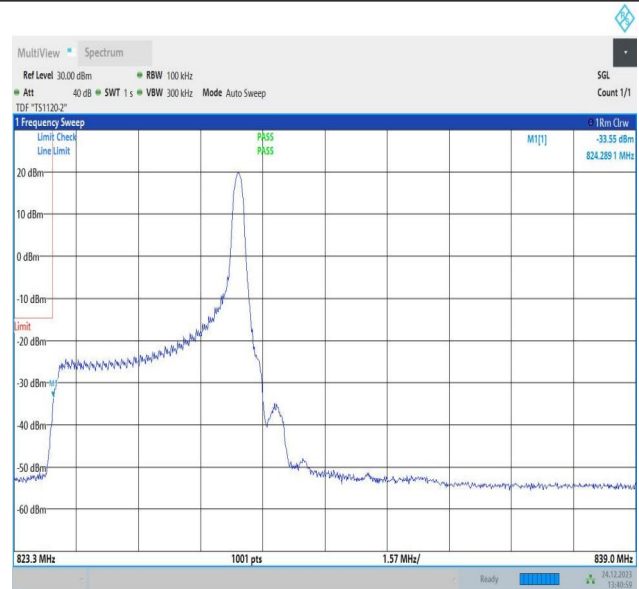
5MHz-10MHz_16QAM@16QAM-16QAM@16QAM_20428-20500_1RB#0@25RB#0-0RB#0@50RB#0
