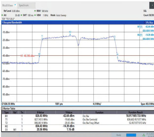
5-5-10MHz-10MHz-QPSK-QPSK-20476-20575-50RB#0-50RB #0-PASS
