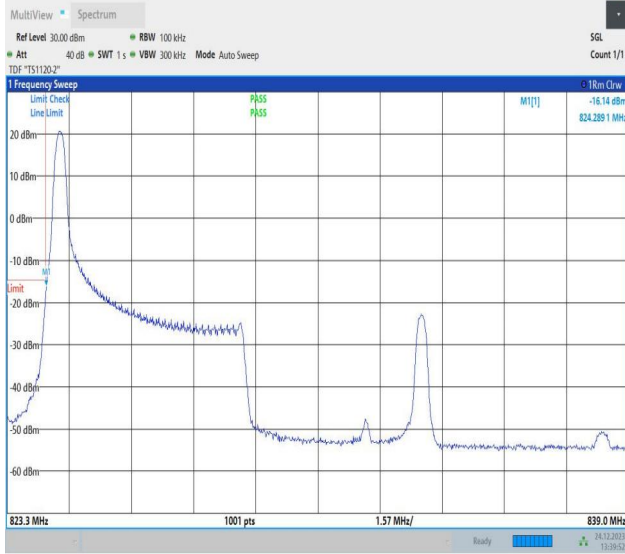
5MHz-10MHz_QPSK@QPSK-QPSK@QPSK_20428-20500_1 RB#0@25RB#0-0RB#0@50RB#0
