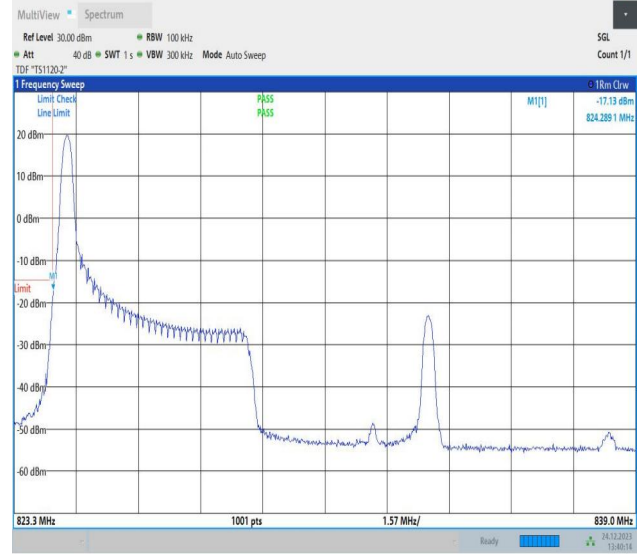
5MHz-10MHz_16QAM@16QAM-16QAM@16QAM_20428-20500_1RB#0@25RB#0-0RB#0@50RB#0
