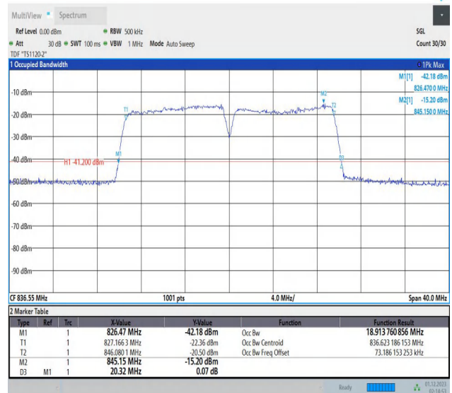
5-5-10MHz-10MHz-16QAM-16QAM-20476-20575-50RB#0-50 RB#0-PASS
