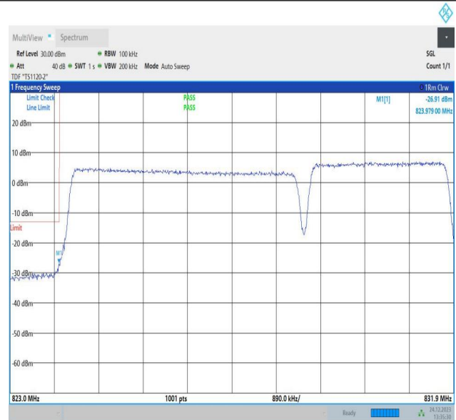
5MHz-3MHz_16QAM@16QAM-16QAM@16QAM_20425-20464_4_1RB#0@25RB#0-1RB#15@15RB#0
