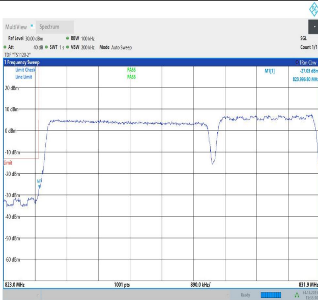
5MHz-3MHz_QPSK@QPSK-QPSK@QPSK_20425-20464_1 RB#0@25RB#0-1RB#15@15RB#0
