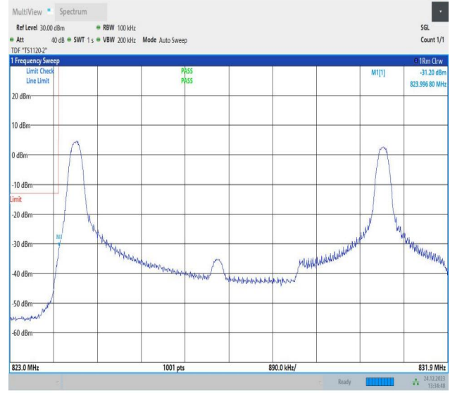
5MHz-3MHz_16QAM@16QAM-16QAM@16QAM_20425-20464_4_1RB#0@25RB#0-1RB#15@15RB#0
