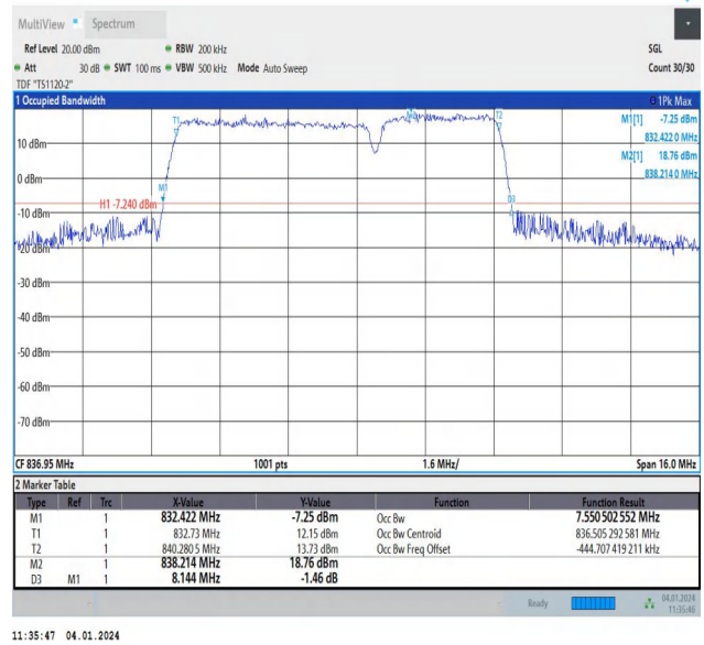
5-5-5MHz-3MHz-64QAM-64QAM-20510-20549-25RB#0-15RB #0-PASS
