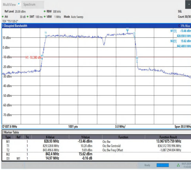
5-5-10MHz-5MHz-64QAM-64QAM-20500-20572-50RB#0-25R B#0-PASS
