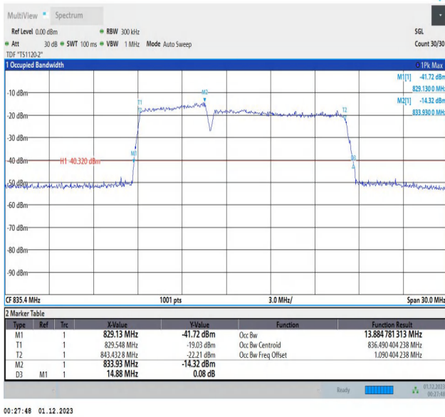
5-5-5MHz-10MHz-QPSK-QPSK-20478-20550-25RB#0-50RB# 0-PASS
