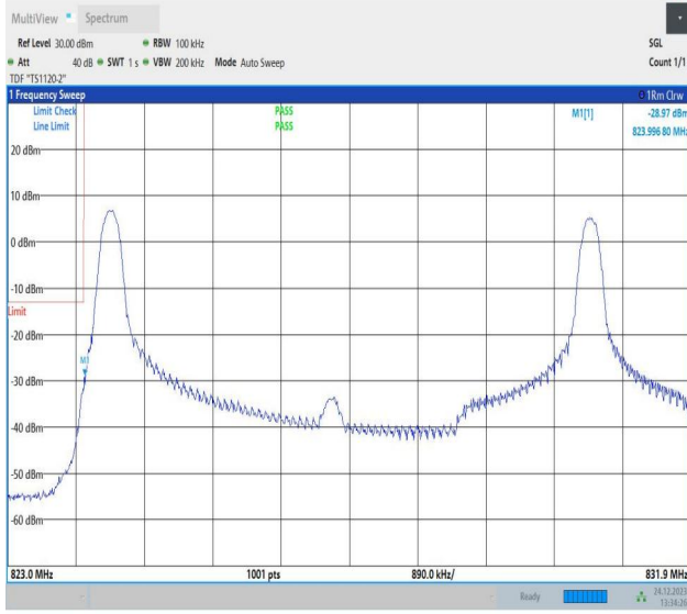
5MHz-3MHz_QPSK@QPSK-QPSK@QPSK_20425-20464_1 RB#0@25RB#0-1RB#15@15RB#0
