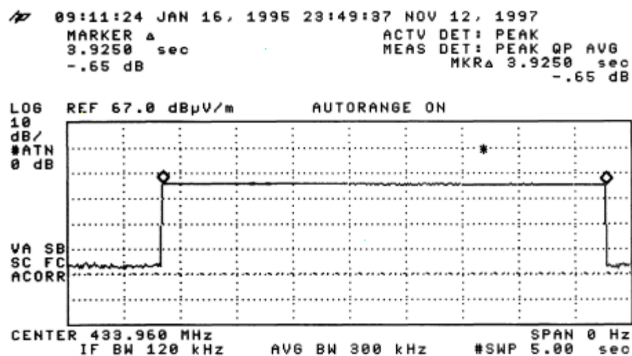
Figure D [Periodic Operation]
