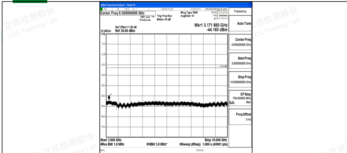
Band5_5MHz_16QAM_20625_1RB#0_3000~10000_3000~10000
