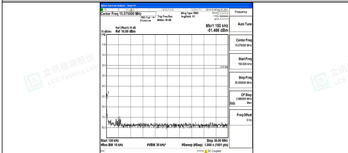
Band5_10MHz_QPSK_20450_1RB#0_0.15~30_0.15~30
