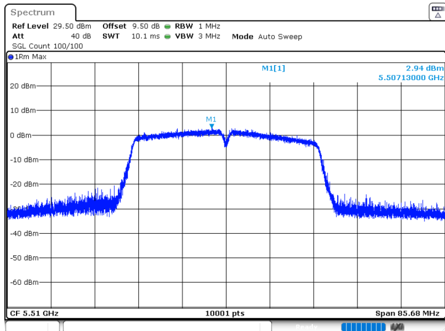
PSD NVNT 802.11ac40 5510MHz Ant1
