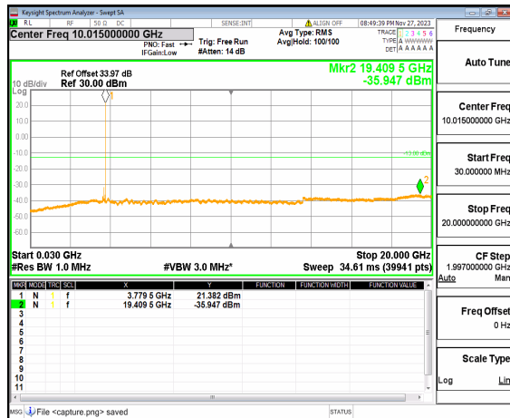
n77(3700-3980MHz) (30MHz-20GHz) 80M DFT-s-OFDM QPSK Edge 1RB Right Low
