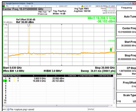
n77(3700-3980MHz) (30MHz-20GHz) 80M DFT-s-OFDM QPSK Edge 1RB Left Mid
