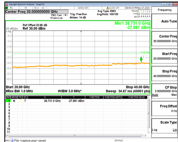
n77(3700-3980MHz) (20GHz-40GHz) 80M DFT-s-OFDM QPSK Edge_1RB_Left_High
