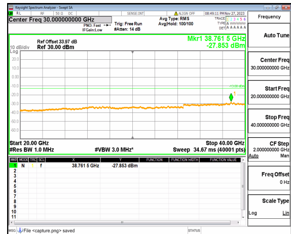
n77(3700-3980MHz) (20GHz-40GHz) 80M DFT-s-OFDM QPSK Edge 1RB Left Low
