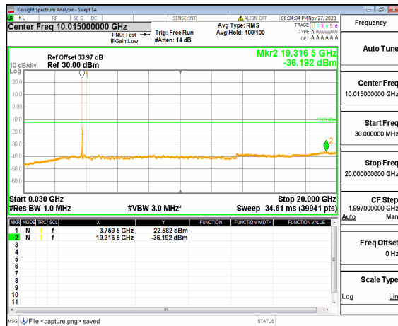
n77(3700-3980MHz) (30MHz-20GHz) 60M DFT-s-OFDM QPSK Edge 1RB Right Low
