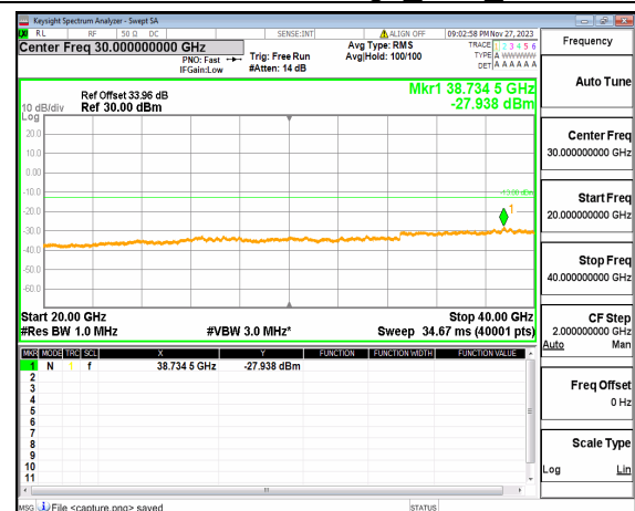
n77(3700-3980MHz) (20GHz-40GHz) 100M DFT-s-OFDM BPSK Edge 1RB Right Low
