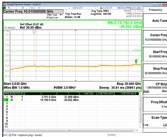
n77(3700-3980MHz) (30MHz-20GHz) 60M DFT-s-OFDM QPSK Edge 1RB Left Low
