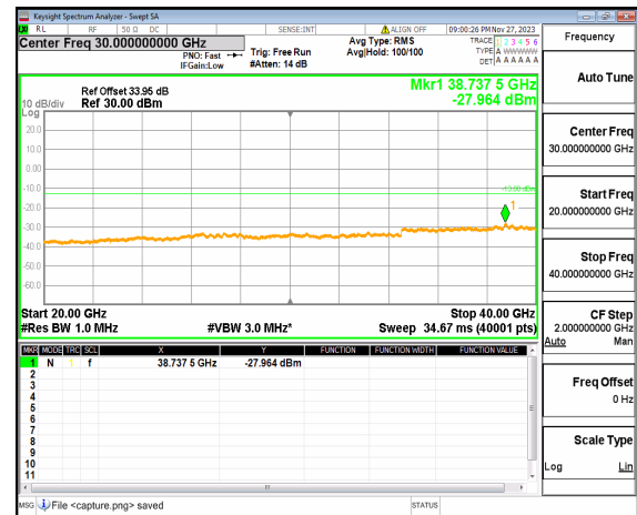
n77(3700-3980MHz) (20GHz-40GHz) 80M DFT-s-OFDM QPSK Edge 1RB Right High
