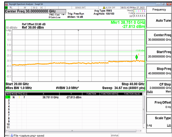
n77(3700-3980MHz) (20GHz-40GHz) 80M DFT-s-OFDM BPSK Edge 1RB Left Mid
