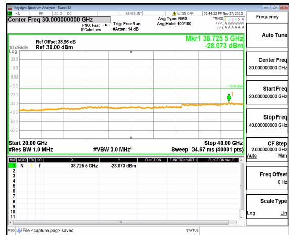
n77(3700-3980MHz) (20GHz-40GHz) 100M DFT-s-OFDM BPSK Edge 1RB Right Mid
