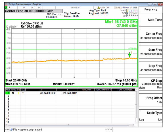
n77(3700-3980MHz) (20GHz-40GHz) 100M DFT-s-OFDM QPSK Edge_1RB_Right High
