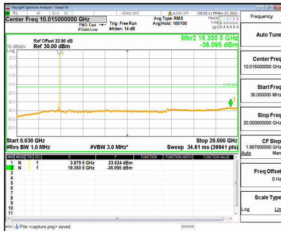
n77(3700-3980MHz) (30MHz-20GHz) 80M DFT-s-OFDM BPSK Edge 1RB Right Mid
