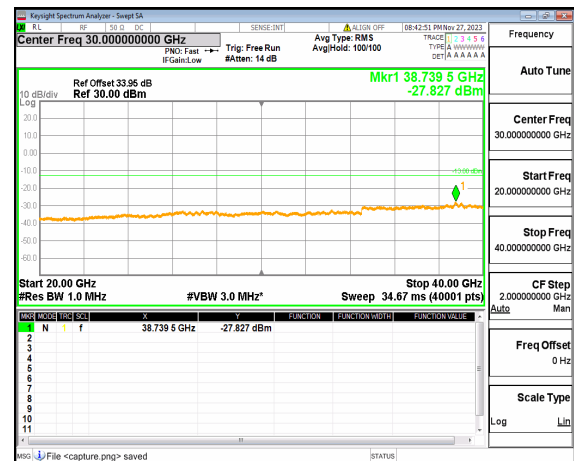
n77(3700-3980MHz) (20GHz-40GHz) 60M DFT-s-OFDM BPSK Edge_1RB_Right_High
