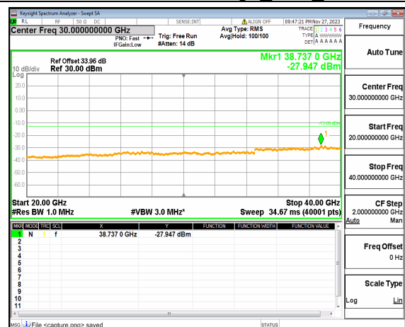
n77(3700-3980MHz) (20GHz-40GHz) 100M DFT-s-OFDM QPSK Edge 1RB Right Mid
