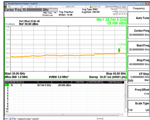
n77(3700-3980MHz) (20GHz-40GHz) 60M DFT-s-OFDM QPSK Edge_1RB_Left_High
