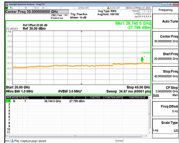
n77(3700-3980MHz) (20GHz-40GHz) 80M DFT-s-OFDM QPSK Edge 1RB Left Mid
