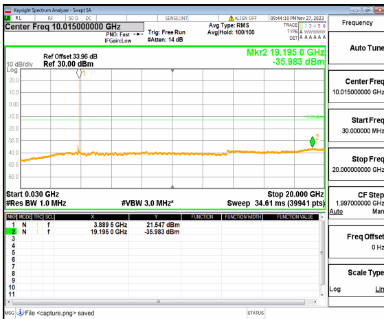
n77(3700-3980MHz) (30MHz-20GHz) 100M DFT-s-OFDM BPSK Edge 1RB Right Mid
