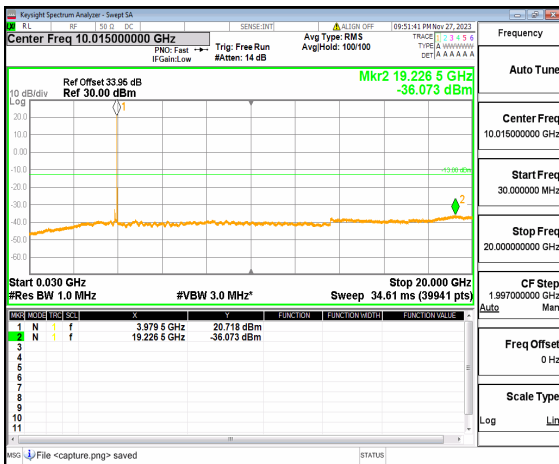
n77(3700-3980MHz) (30MHz-20GHz) 100M DFT-s-OFDM QPSK Edge_1RB_Right High
