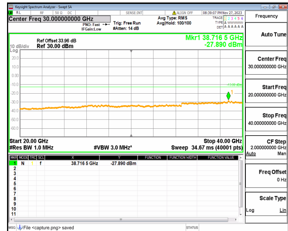
n77(3700-3980MHz) (20GHz-40GHz) 60M DFT-s-OFDM QPSK Edge 1RB Left Mid
