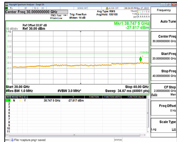
n77(3700-3980MHz) (20GHz-40GHz) 60M DFT-s-OFDM QPSK Edge 1RB Left Low
