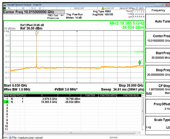
n77(3700-3980MHz) (30MHz-20GHz) 60M DFT-s-OFDM BPSK Edge_1RB_Right_High
