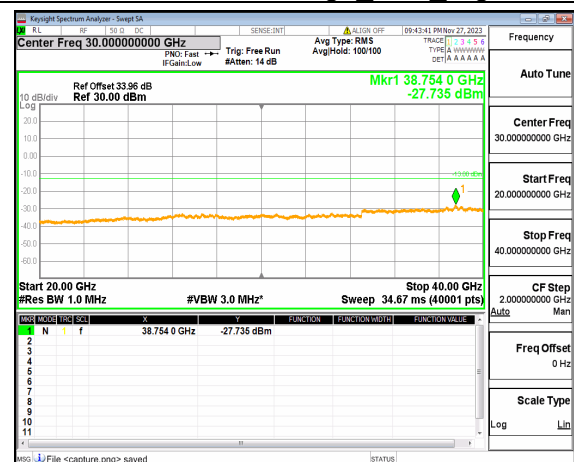
n77(3700-3980MHz) (20GHz-40GHz) 100M DFT-s-OFDM BPSK Edge 1RB Left Mid
