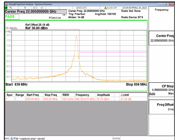
n5 10M DFT-s-OFDM BPSK Edge_1RB_Right High
