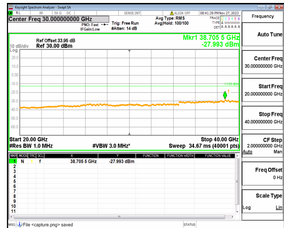
n77(3700-3980MHz) (20GHz-40GHz) 60M DFT-s-OFDM BPSK Edge_1RB_Left_High
