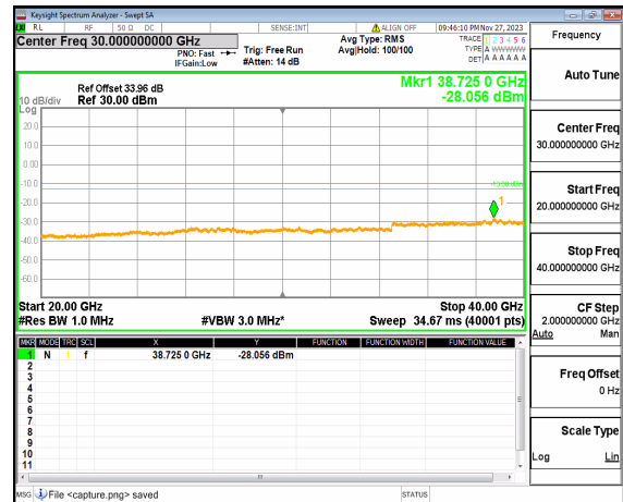
n77(3700-3980MHz) (20GHz-40GHz) 100M DFT-s-OFDM QPSK Edge 1RB Left Mid
