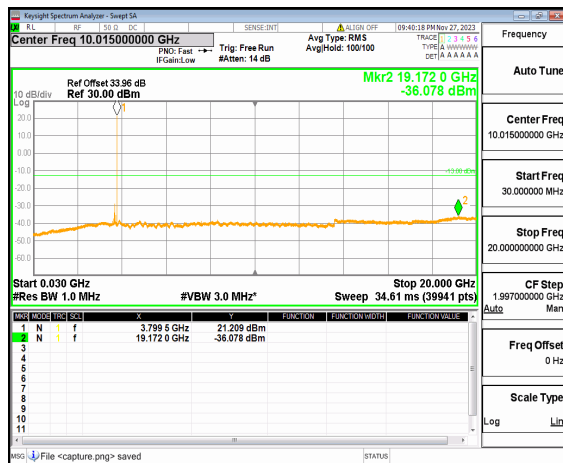
n77(3700-3980MHz) (30MHz-20GHz) 100M DFT-s-OFDM QPSK Edge 1RB Right Low
