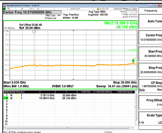
n77(3700-3980MHz) (30MHz-20GHz) 100M DFT-s-OFDM BPSK Edge 1RB Left Mid
