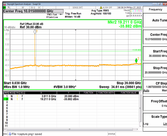
n77(3700-3980MHz) (30MHz-20GHz) 60M DFT-s-OFDM QPSK Edge 1RB Left Mid
