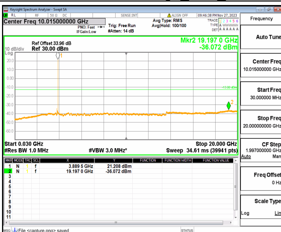
n77(3700-3980MHz) (30MHz-20GHz) 100M DFT-s-OFDM QPSK Edge 1RB Right Mid
