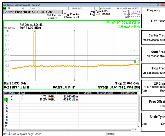
n77(3700-3980MHz) (30MHz-20GHz) 100M DFT-s-OFDM QPSK Edge 1RB Left Low
