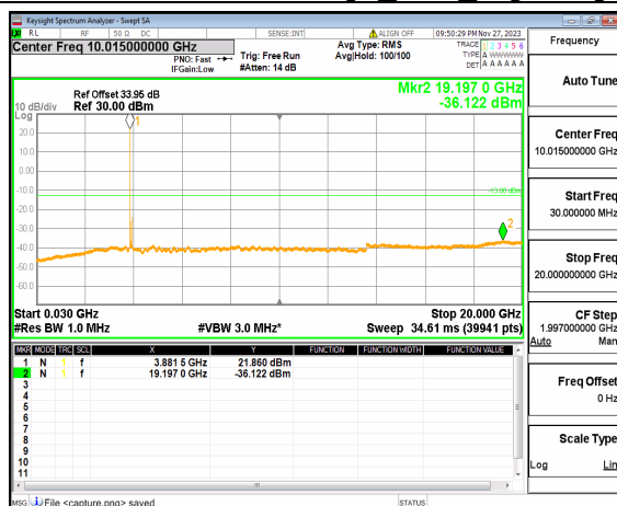
n77(3700-3980MHz) (30MHz-20GHz) 100M DFT-s-OFDM QPSK Edge_1RB_Left_High
