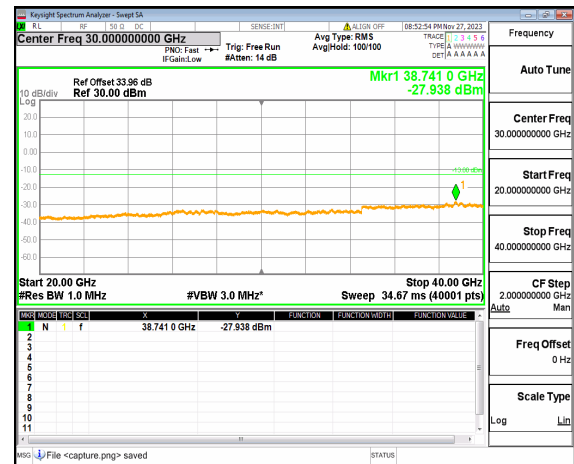
n77(3700-3980MHz) (20GHz-40GHz) 80M DFT-s-OFDM BPSK Edge 1RB Right Mid
