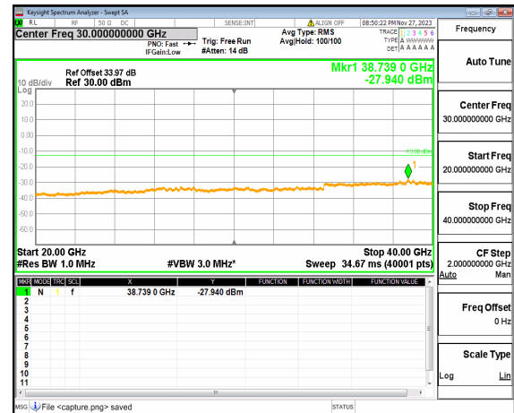
n77(3700-3980MHz) (20GHz-40GHz) 80M DFT-s-OFDM QPSK Edge 1RB Right Low
