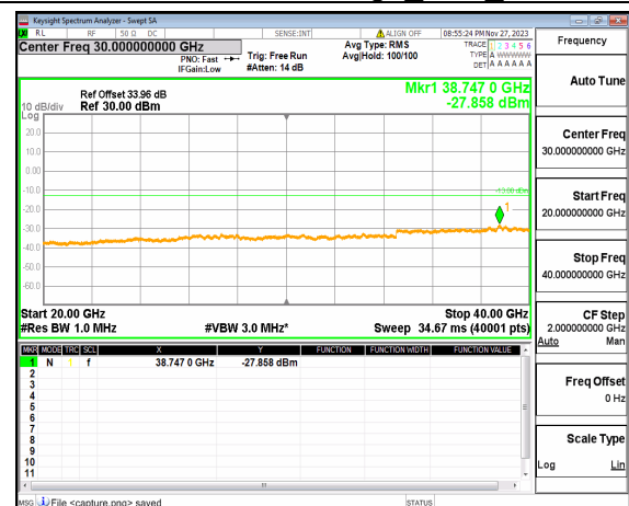
n77(3700-3980MHz) (20GHz-40GHz) 80M DFT-s-OFDM QPSK Edge 1RB Right Mid
