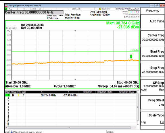
n77(3700-3980MHz) (20GHz-40GHz) 60M DFT-s-OFDM QPSK Edge 1RB Right Mid
