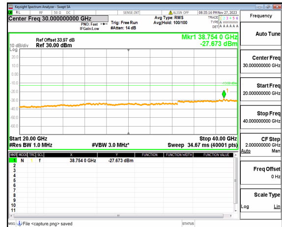
n77(3700-3980MHz) (20GHz-40GHz) 60M DFT-s-OFDM QPSK Edge 1RB Right Low
