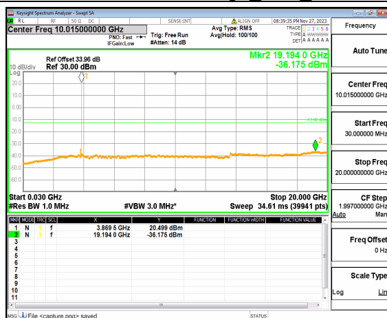
n77(3700-3980MHz) (30MHz-20GHz) 60M DFT-s-OFDM QPSK Edge 1RB Right Mid
