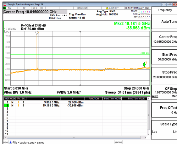
n77(3700-3980MHz) (30MHz-20GHz) 80M DFT-s-OFDM BPSK Edge 1RB Left Mid
