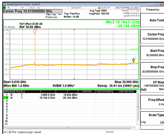
n77(3700-3980MHz) (30MHz-20GHz) 60M DFT-s-OFDM BPSK Edge 1RB Right Mid
