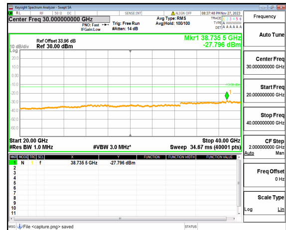
n77(3700-3980MHz) (20GHz-40GHz) 60M DFT-s-OFDM BPSK Edge 1RB Right Mid
