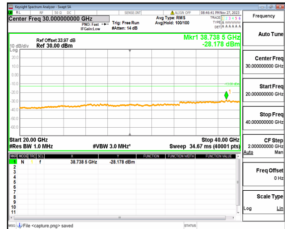
n77(3700-3980MHz) (20GHz-40GHz) 80M DFT-s-OFDM BPSK Edge_1RB_Left_Low
