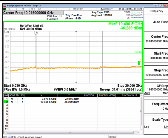
n77(3700-3980MHz) (30MHz-20GHz) 80M DFT-s-OFDM QPSK Edge 1RB Right Mid
