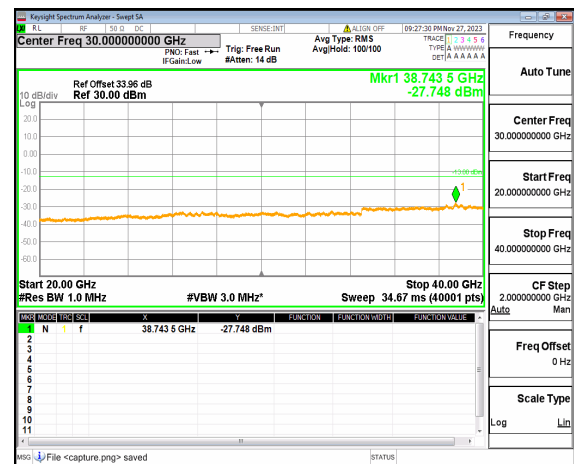
n77(3700-3980MHz) (20GHz-40GHz) 100M DFT-s-OFDM QPSK Edge 1RB Left Low
