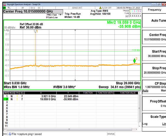
n77(3700-3980MHz) (30MHz-20GHz) 60M DFT-s-OFDM BPSK Edge_1RB_Left_High
