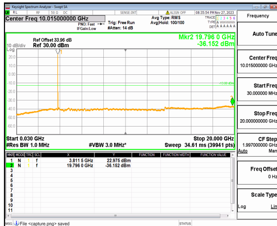
n77(3700-3980MHz) (30MHz-20GHz) 60M DFT-s-OFDM BPSK Edge 1RB Left Mid
