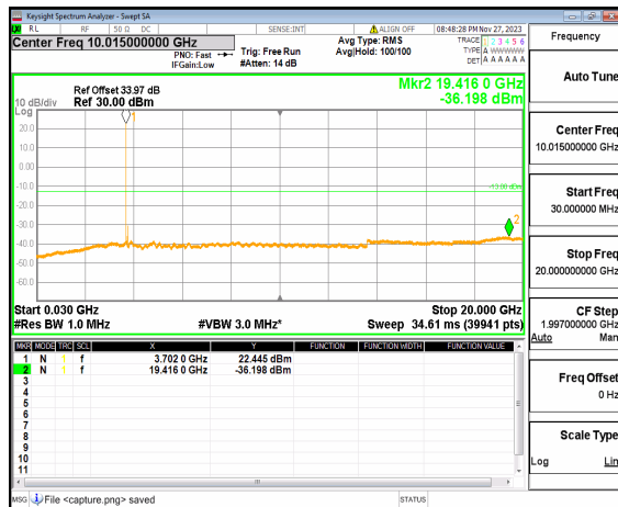
n77(3700-3980MHz) (30MHz-20GHz) 80M DFT-s-OFDM QPSK Edge 1RB Left Low
