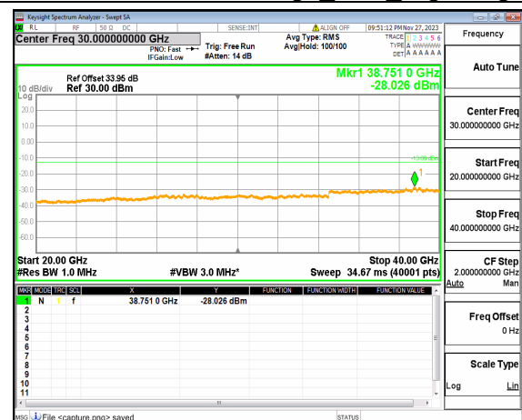
n77(3700-3980MHz) (20GHz-40GHz) 100M DFT-s-OFDM QPSK Edge_1RB_Left_High
