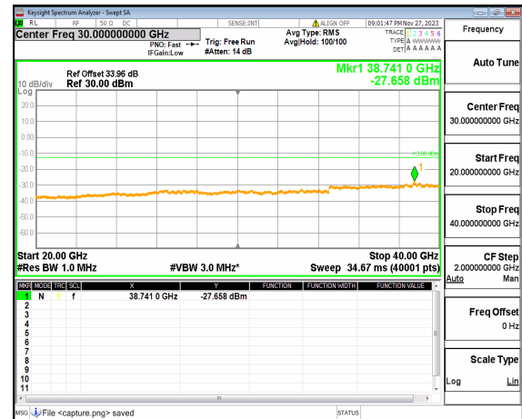
n77(3700-3980MHz) (20GHz-40GHz) 100M DFT-s-OFDM BPSK Edge 1RB Left Low
