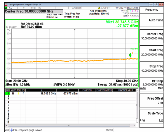
n77(3700-3980MHz) (20GHz-40GHz) 100M DFT-s-OFDM QPSK Edge 1RB Right Low
