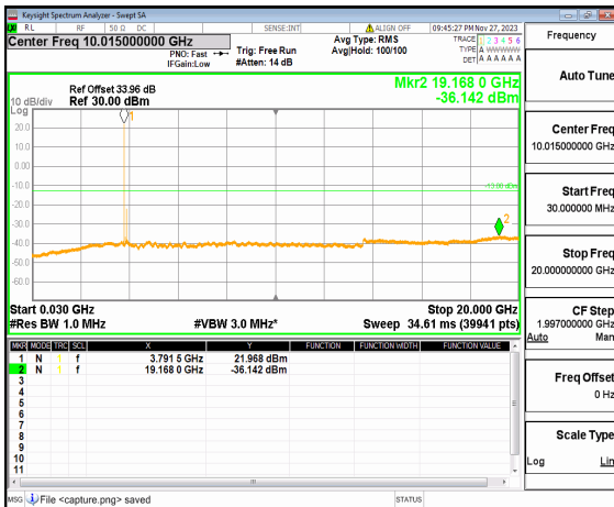
n77(3700-3980MHz) (30MHz-20GHz) 100M DFT-s-OFDM QPSK Edge 1RB Left Mid
