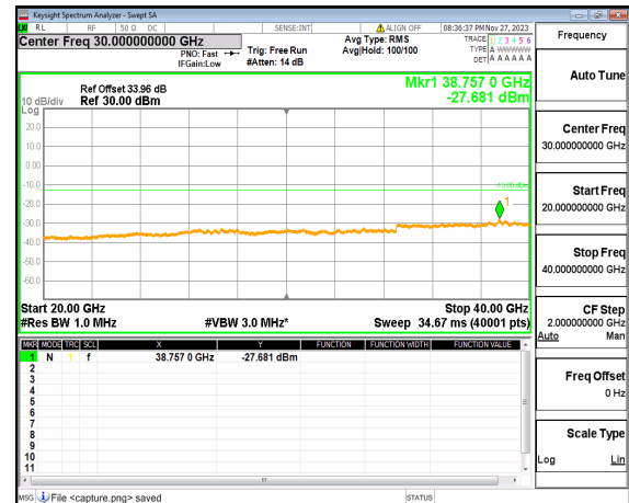
n77(3700-3980MHz) (20GHz-40GHz) 60M DFT-s-OFDM BPSK Edge 1RB Left Mid
