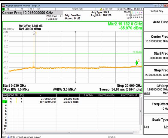
n77(3700-3980MHz) (30MHz-20GHz) 100M DFT-s-OFDM BPSK Edge 1RB Right Low
