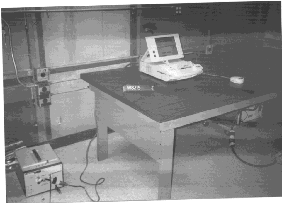
Test-setup photo(s): Conducted emission 10/150 kHz - 30 MHz
